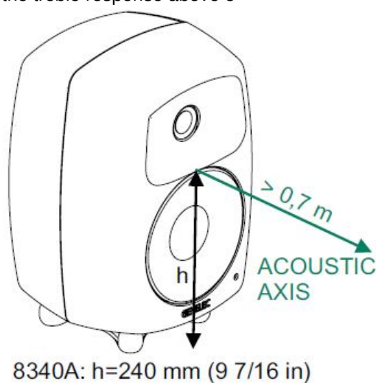
Figure 3. The location of the acoustic axis is on the center-line of the monitor at the given height “h”.
