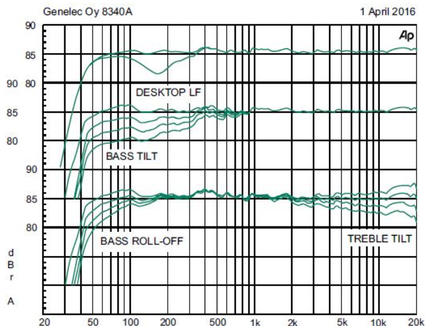
Figure 7. The curves above show the effect of the “Bass Tilt”, “Treble Tilt”, “Desktop Low Frequency” and “Bass Roll-Off” controls on the free field response of the 8340A.
