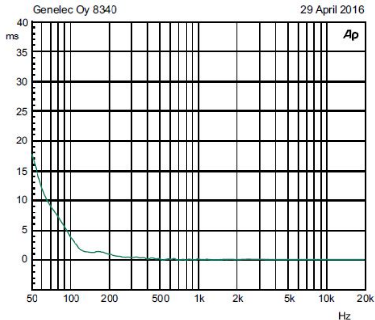
Figure 9. The curve above shows the delay variation of the 8340A as a function of frequency.
