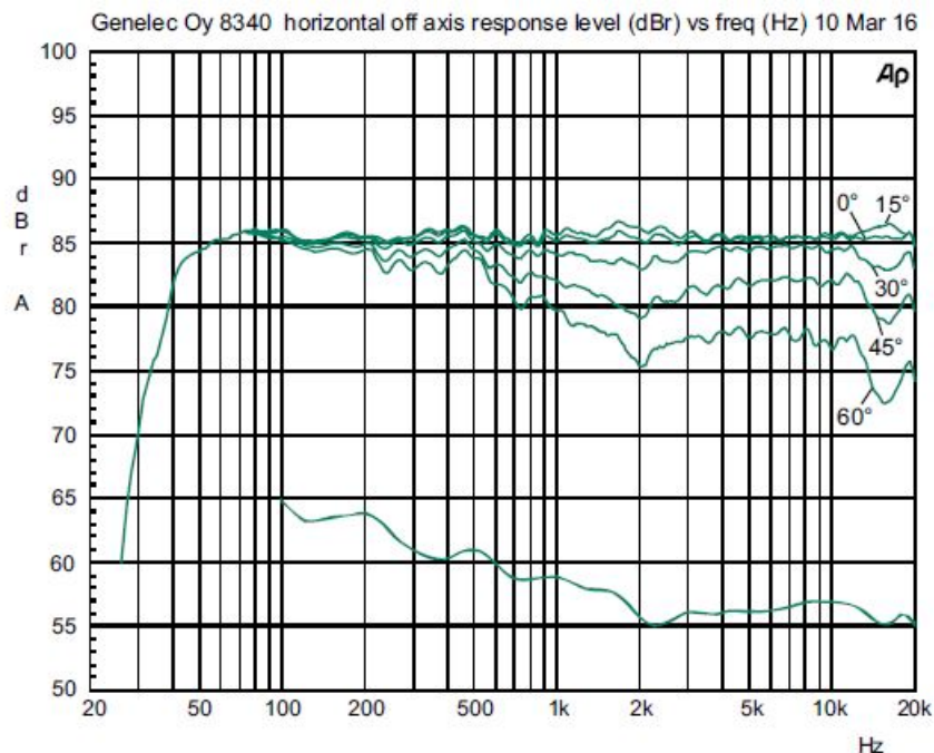
Figure 8. The upper curve group shows the horizontal directivity characteristics of the 8340A measured at 1 m. The lower curve shows the system's power response.
