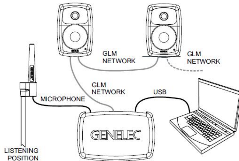
Figure 1. GLM control network cabling
