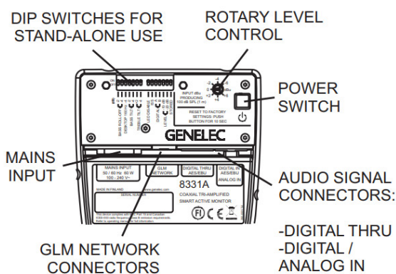
Figure 2. Connectors and controls on the back panel of a 8331A.
