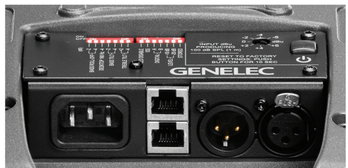
Figure 3. Connector panel detail.
