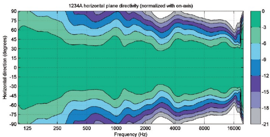
Figure 10. Horizontal directivity characteristics of the 1234A.
