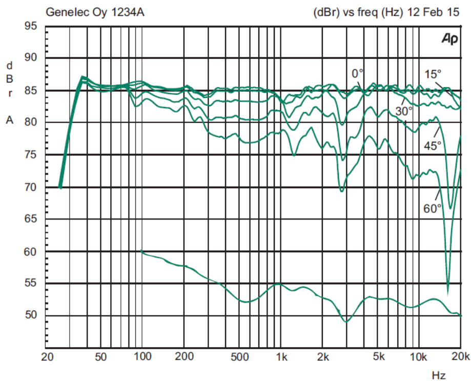
Figure 11. Horizontal directivity characteristics of the 1234A. The lower curve is the monitor’s power response.
