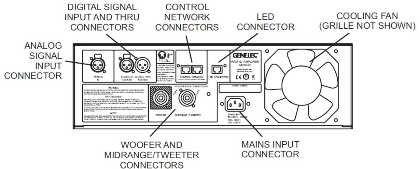
Figure 8. Connector panel of the RAM-XL amplifier.
