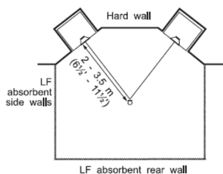
Figure 3. Monitor enclosure mounting details.
