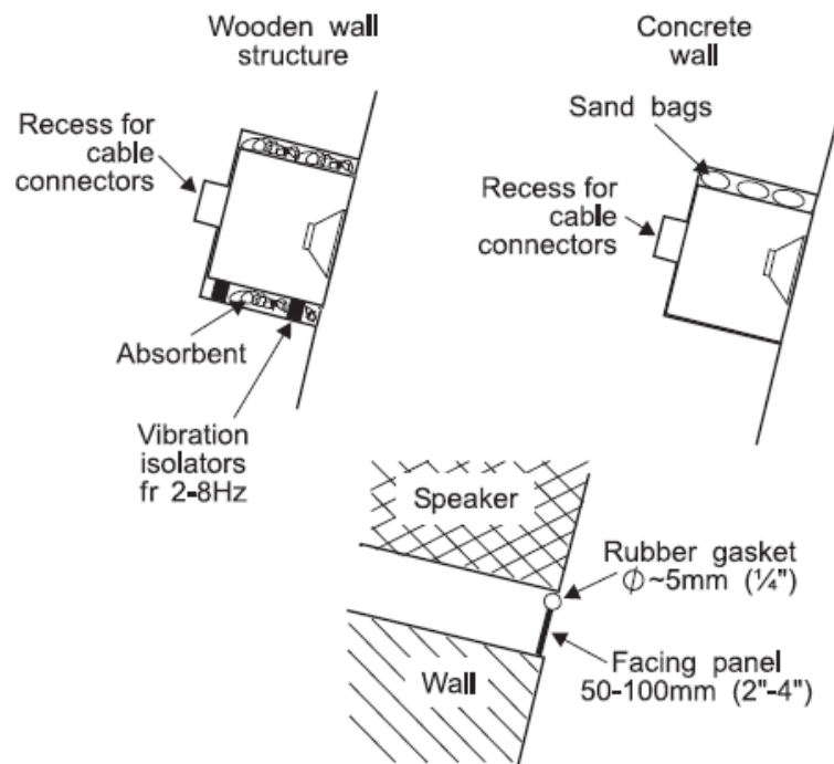
Figure 4. Eliminating discontinuities.
