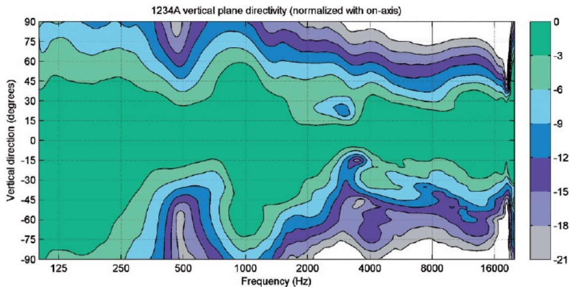
Figure 9. Vertical directivity characteristics of the 1234A.
