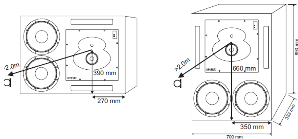
Figure 2. Monitor enclosure mounting.
