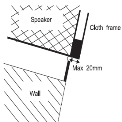
Figure 5. Recess for speaker cable connectors (front view).
