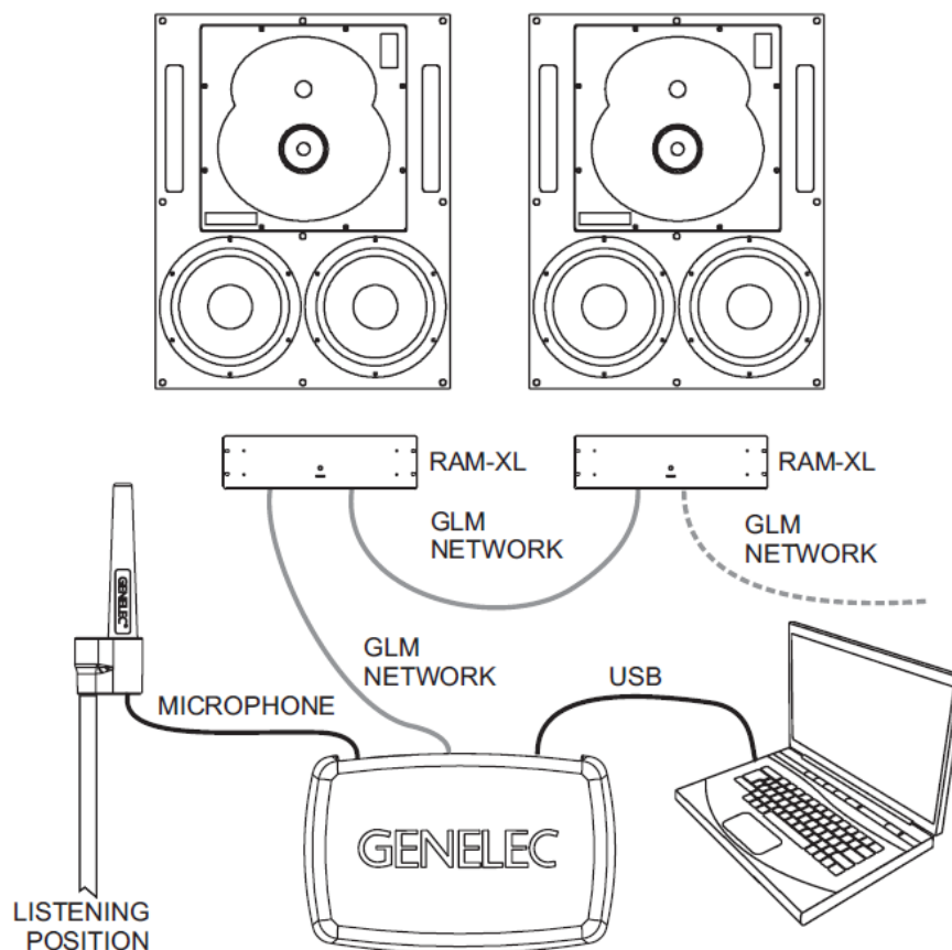
Figure 6. GLM network cabling (audio cabling not shown)
