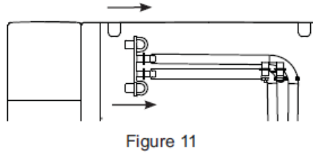
Replace drain tubes
