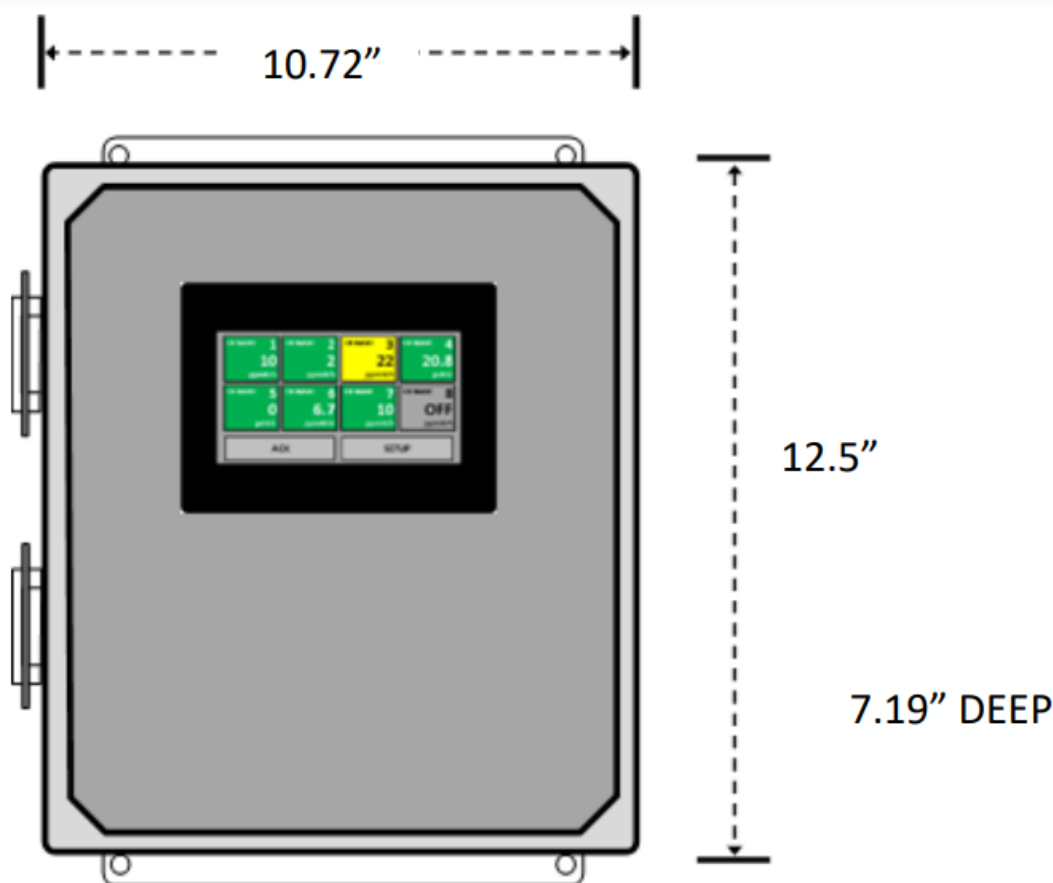
Figure 7-1: Outside Dimensions
