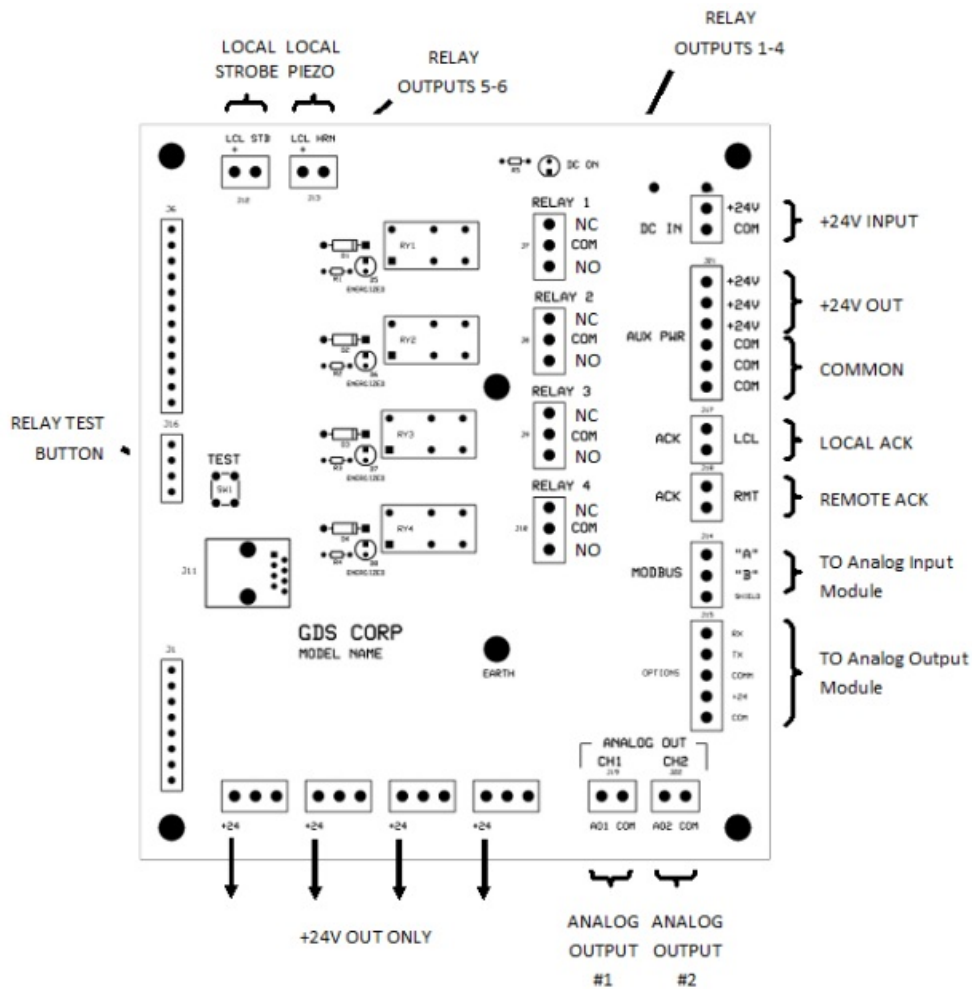
Figure 3-4: P8XA Signal & Relay Connections
