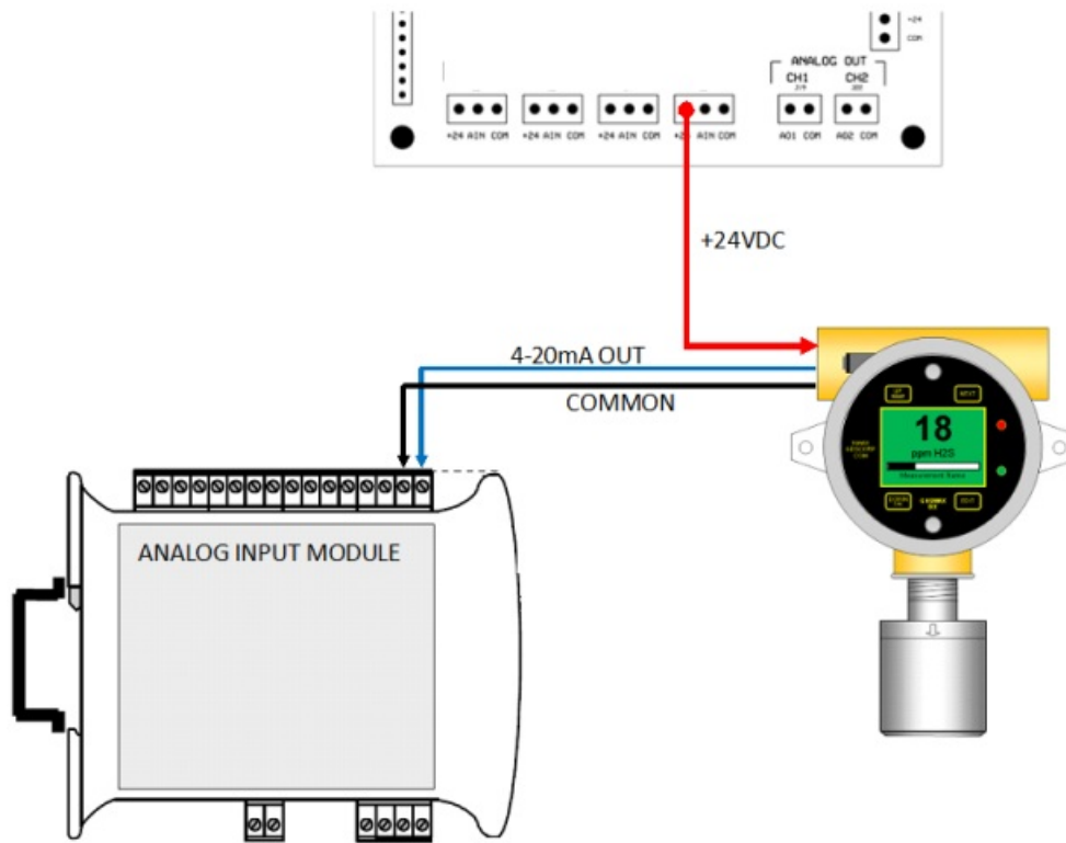
Figure 3-6: Example Sensor Connection (Channel 1)
