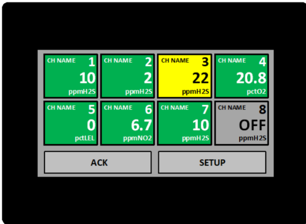
Figure 4-1: Primary Display Screen
