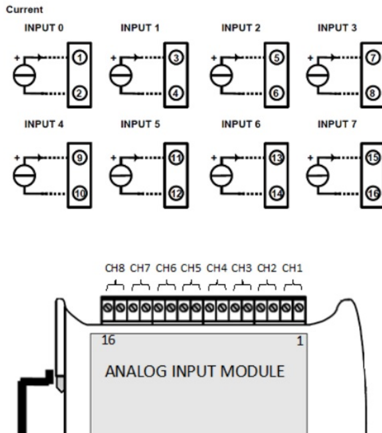
Figure 3-5: P8XA Analog Input Connections
