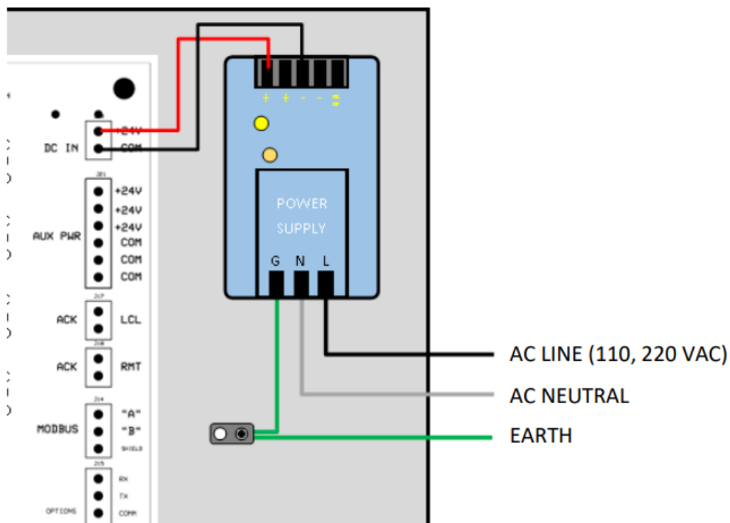
Figure 3-2: AC Power Supply Connections
