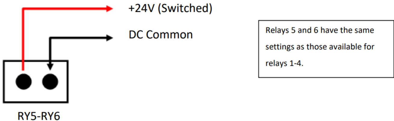
Figure 3-9: Alarm Relay 5-6 Wiring
