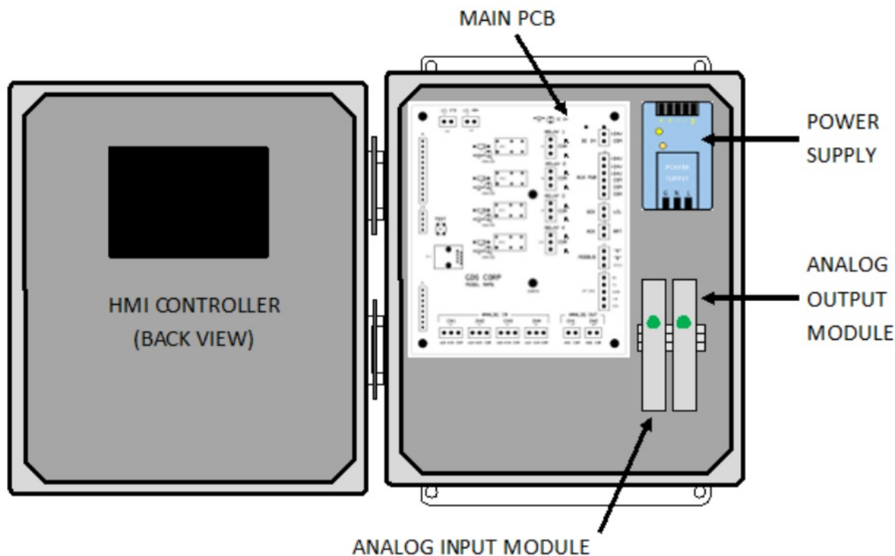
Figure 3-1: P8XA Component Layout
