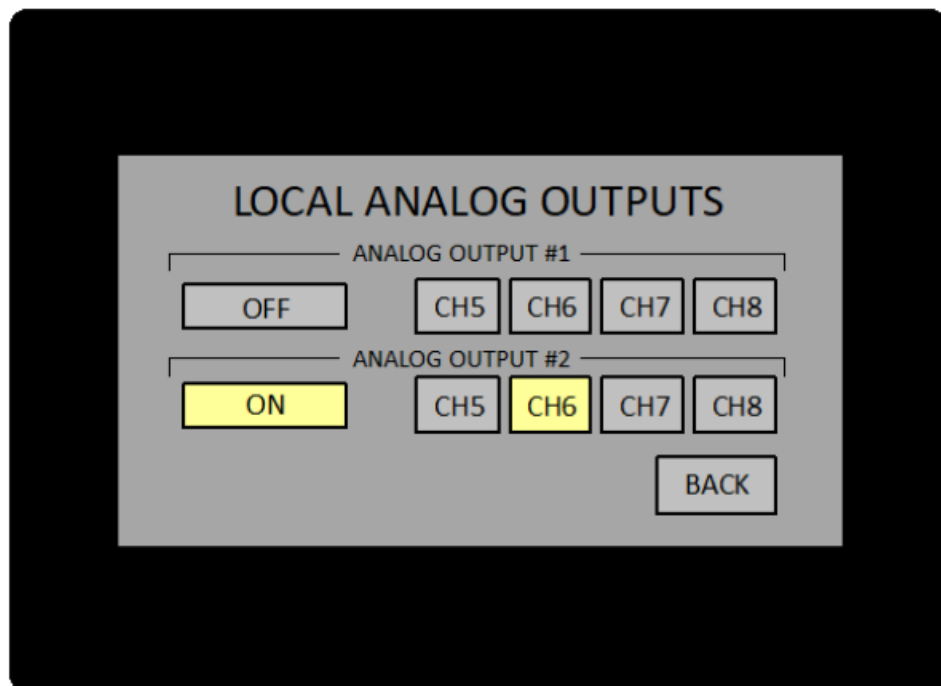
Figure 4-5: Analog Output Screen
