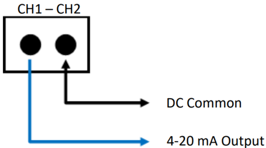
Figure 3-7: Local Analog Output Wiring
