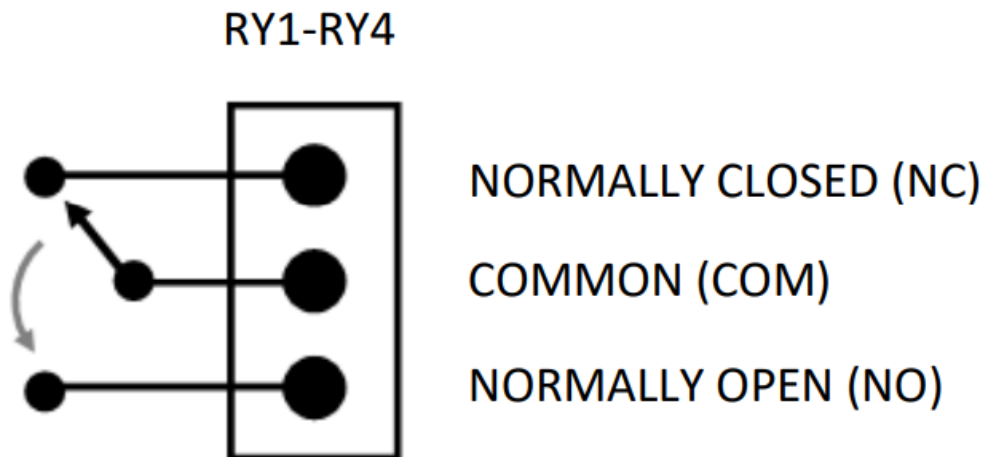
Figure 3-8: Alarm Relay 1-4 Wiring
