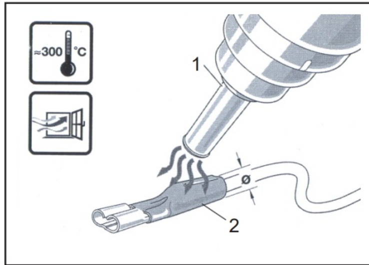
1.Reduction Nozzle 2.Heat-shrinkzble Tubing
