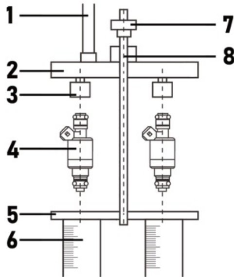
Top-in fuel injector installation diagram
