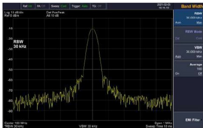
Figure 3-9 Set frequency span
