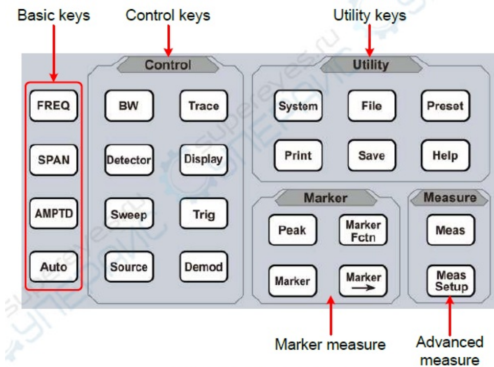
Figure 3-2 Function Keys
