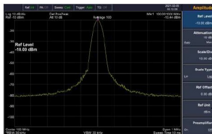
Figure 3-10 Set reference level
