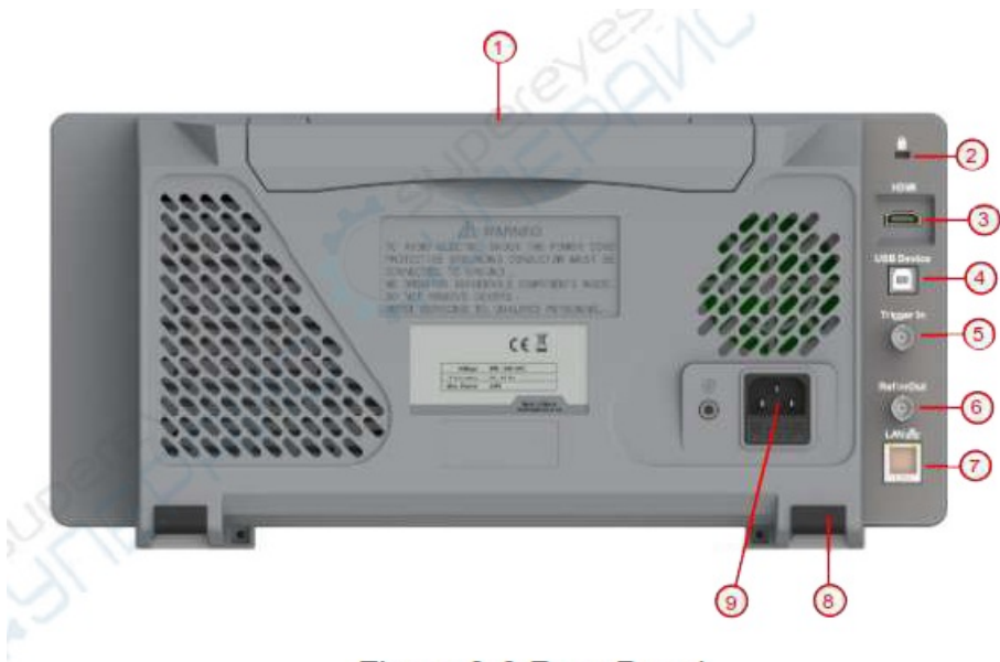
Figure 3-6 Rear Panel
