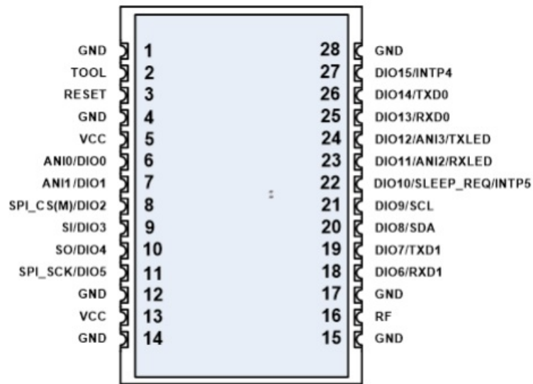
Figure 3-1 Module pin connection diagram
