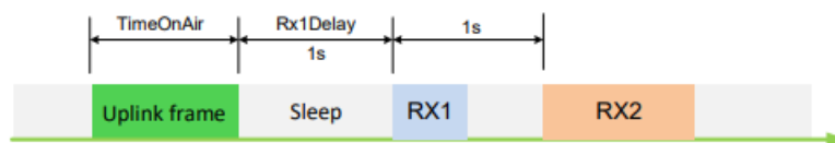
Figure 4-8 Schematic diagram of CLASS A device communication mechanism
