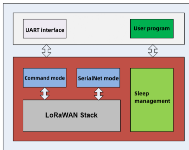
Figure 4-1 Module functional block diagram
