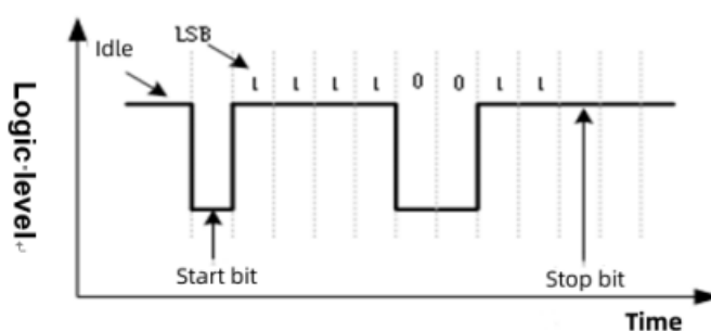
Figure 4-3 Serial communication timing diagram
