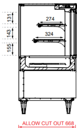
SECTION VIEW
