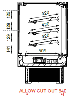
SECTION VIEW
