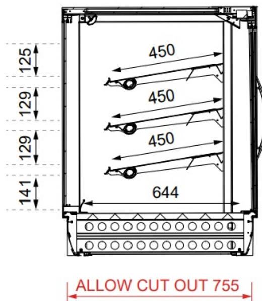
FRONT ELEVATION
