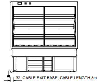
REAR ELEVATION
