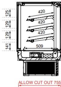
SECTION VIEW
