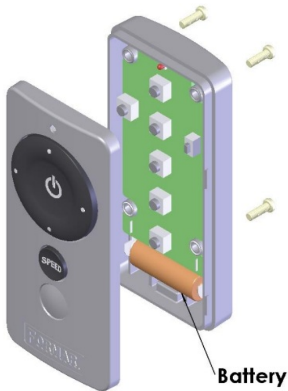
Fig. 3 Battery Location in Remote Controller
