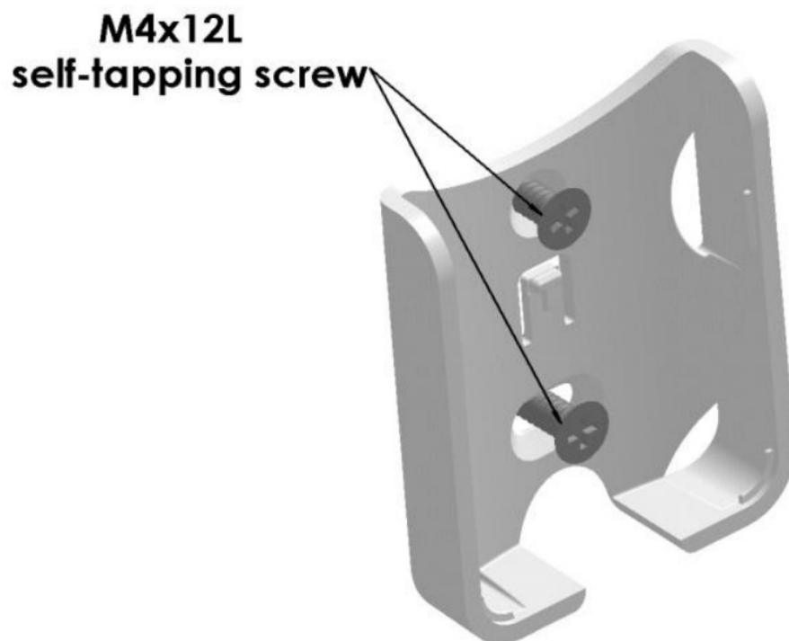
Fig. 1 Installation of Remote Controller mounting bracket
