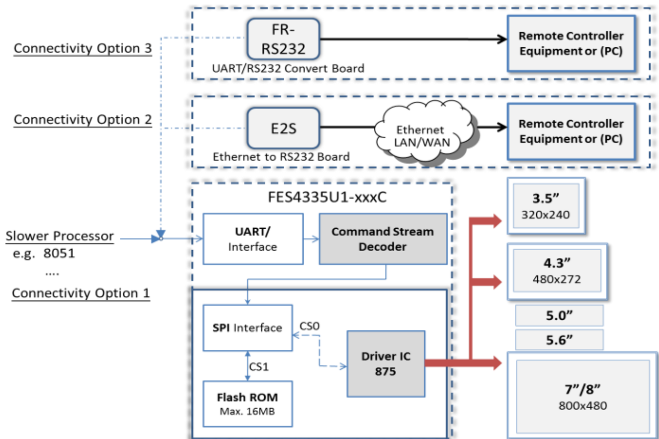
Figure 3-a : The Block Diagram of FES4335U1-xxC
