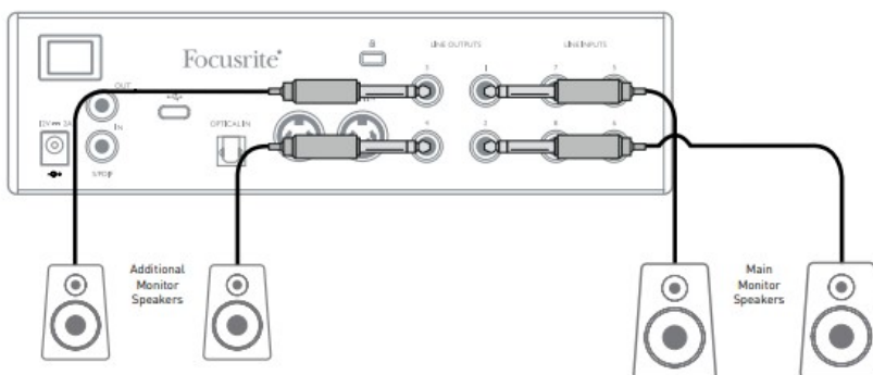
Connecting active speakers
