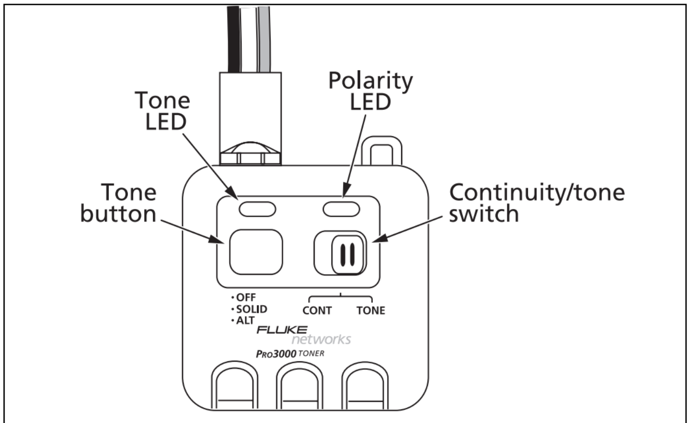
Figure 2. PRO3000 Toner
