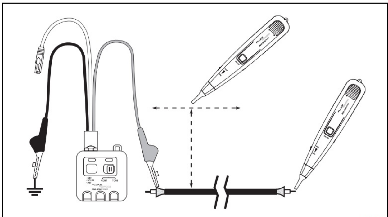
Figure 3. Tracing Cables
