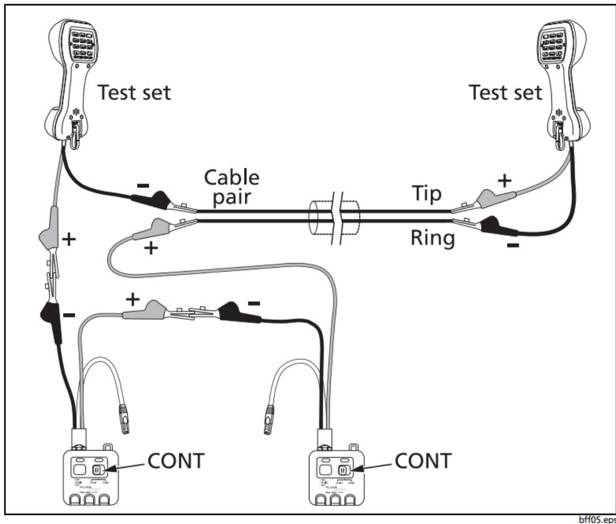
Figure 5. Talk Battery
