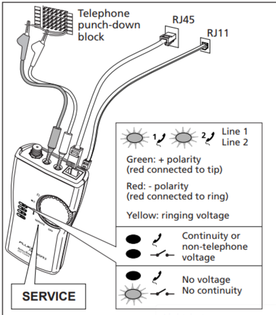
Figure 3. Validating Telephone Service and Polarity
