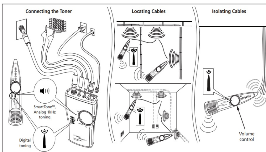
Figure 1. Locating and Isolating Cables
