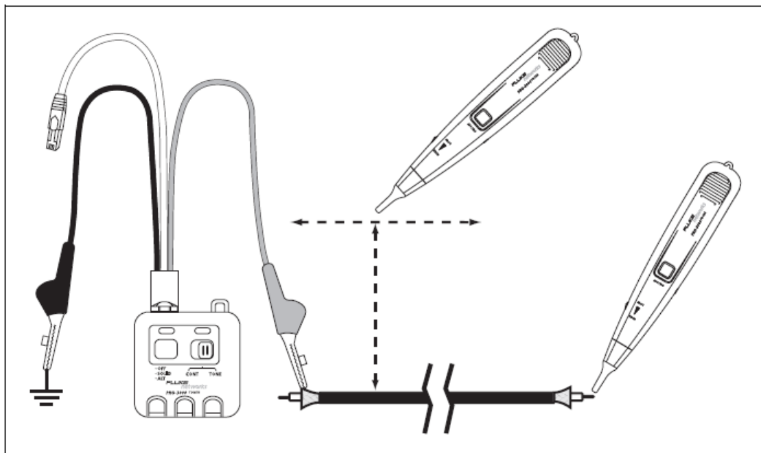
Figure 3. Tracing Cables
