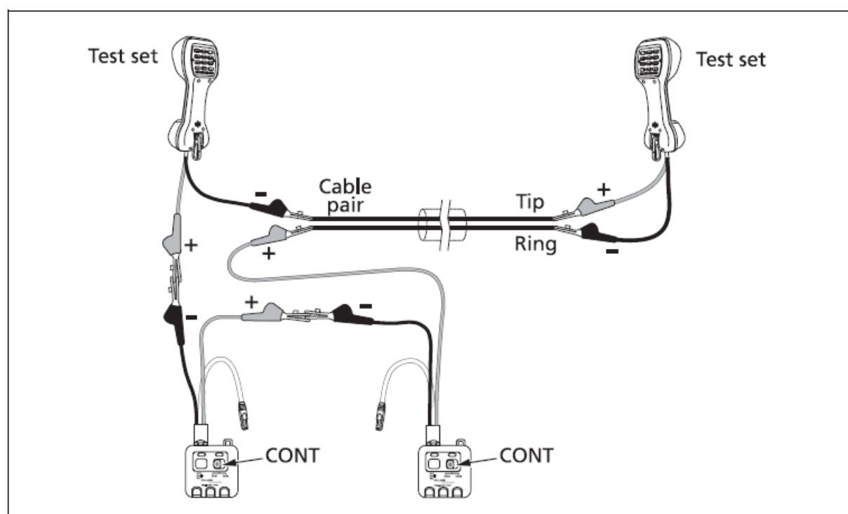
Figure 5. Talk Battery
