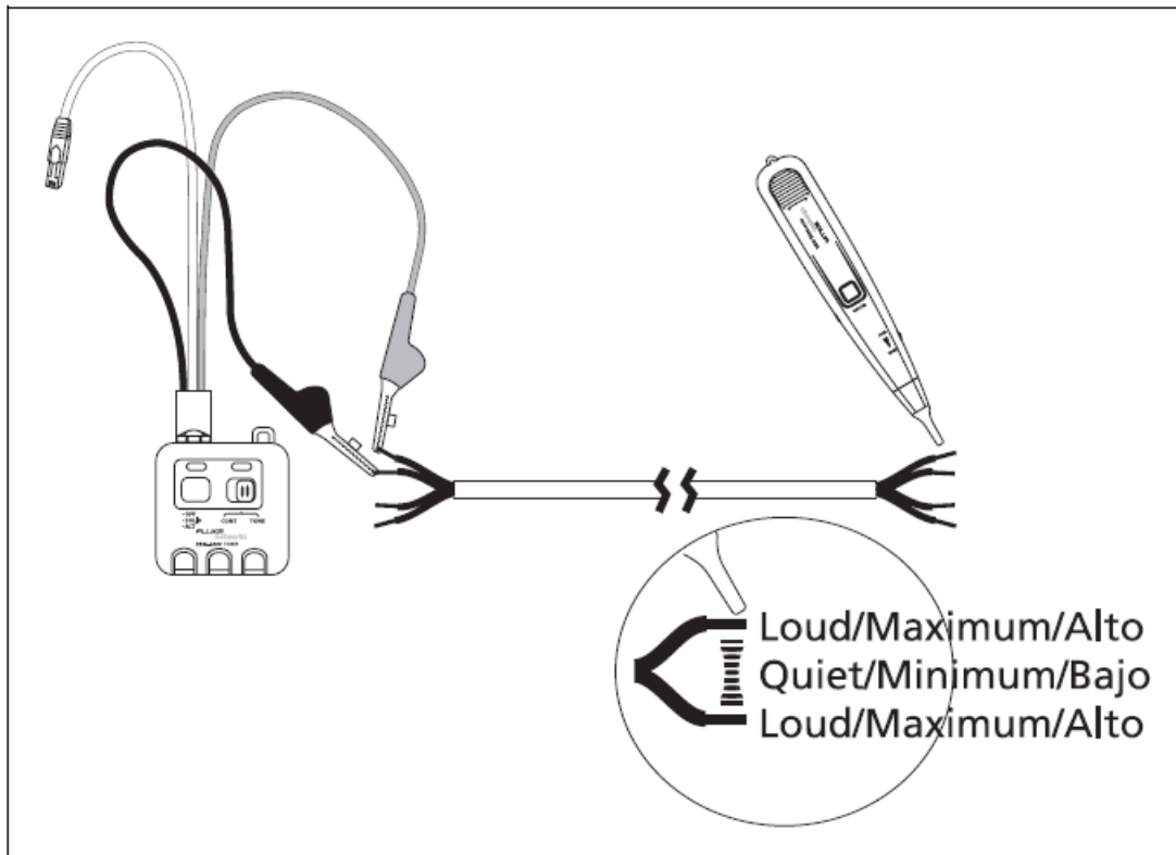
Figure 4. Tracing Pairs
