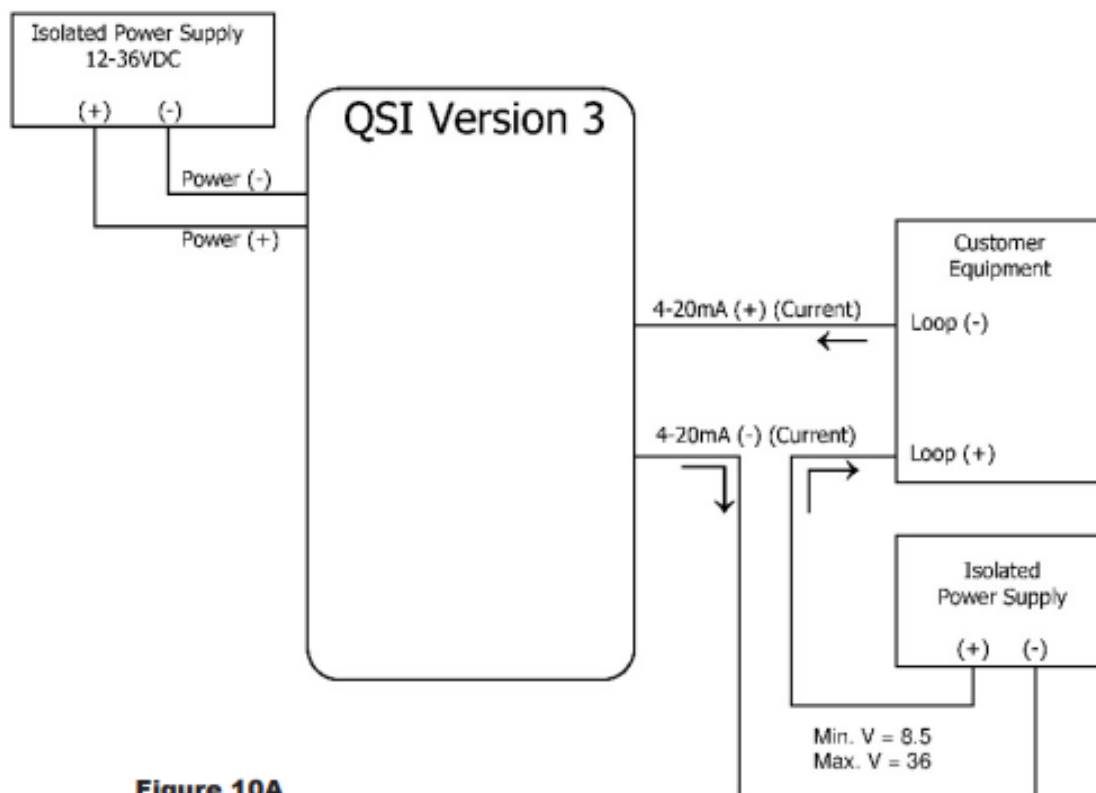
Figure 10A Low Side (Negative) Wiring
