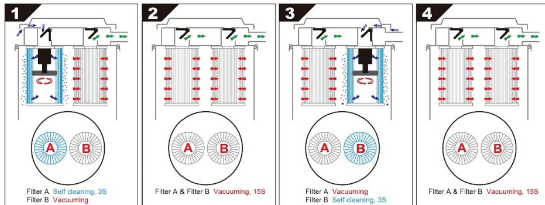
Filter cleaning switch
