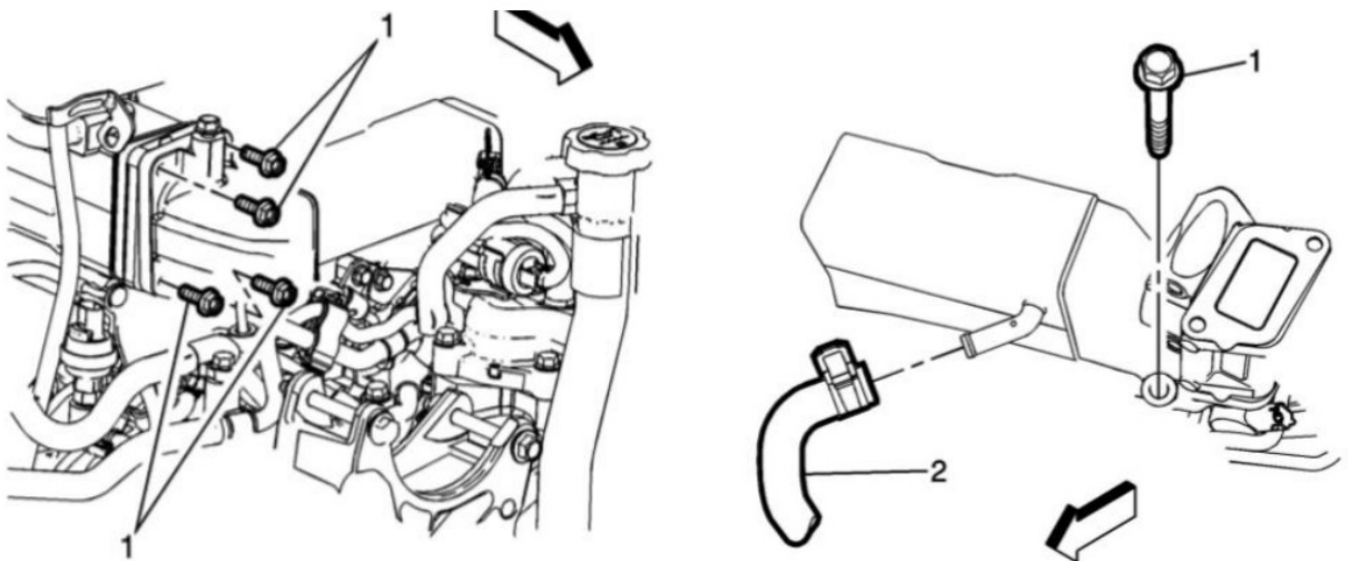
Fig. 5: EGR cooler removal
