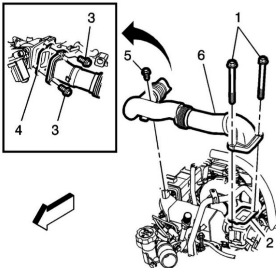
Fig. 3: EGR bypass pipe
