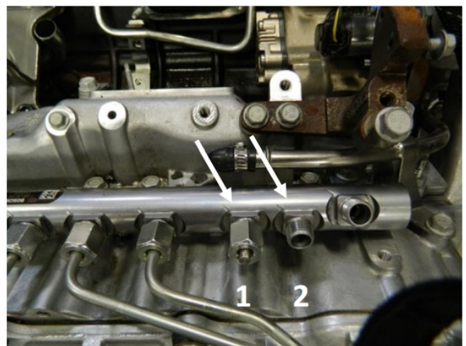
Fuel rail nut (1) and high-pressure line (2)
