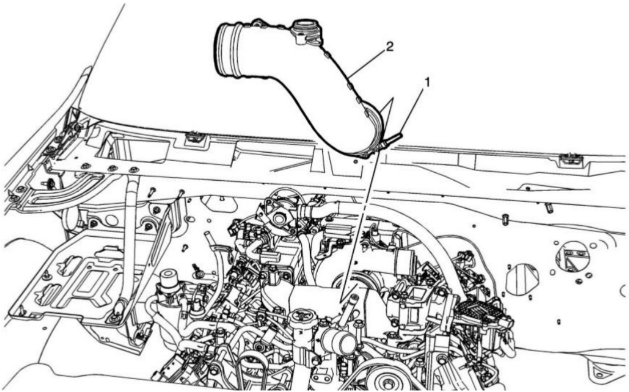
Fig. 2: Air inlet adapter removal
