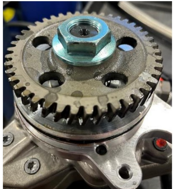
Fig. 12: Install the CP4 nut onto the CP3
