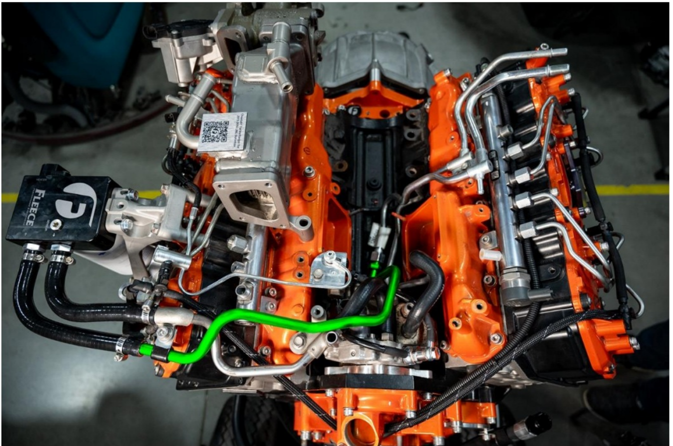
Fuel Feed Hose: Item 2 in kit
