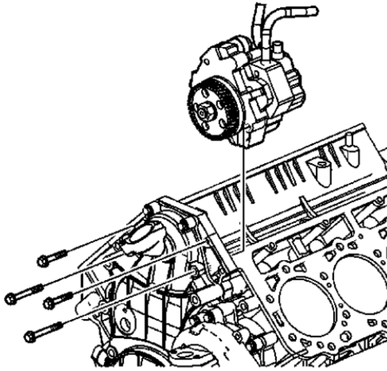
Fig. 10: Remove the CP4 pump
