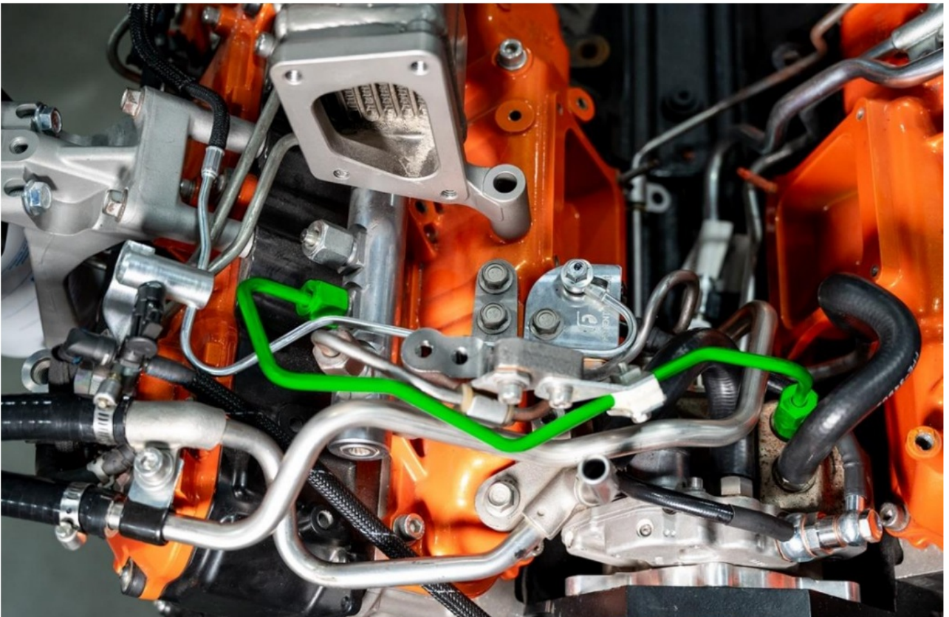
Cascade Return and Feed Lines: Items 14 and 15 in kit OE Dosing Injector Feed Line reused
