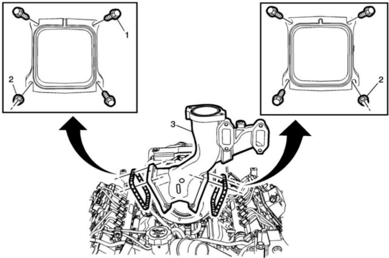
Fig. 6: Turbocharger air inlet removal
