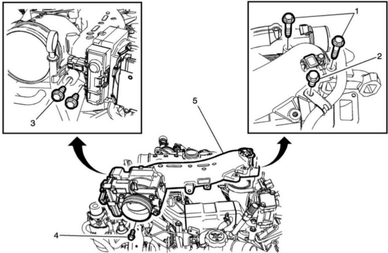
Fig. 1: Intake manifold tube
