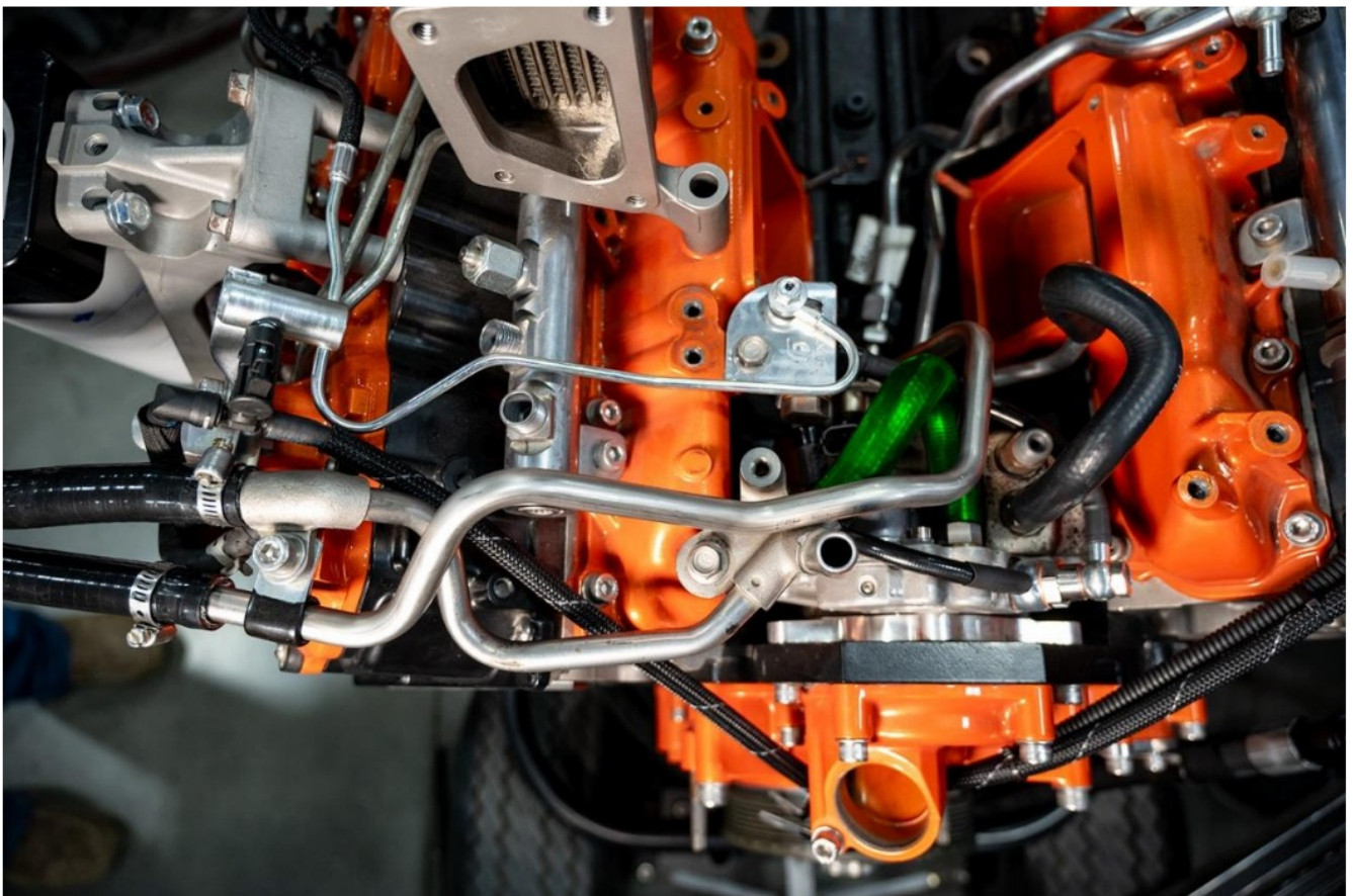
Fuel Return Hose: Item 3 in kit
