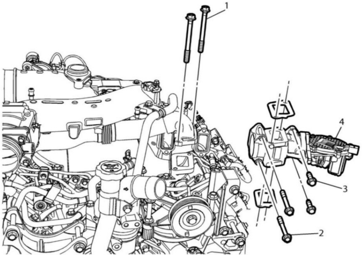
Fig. 4: EGR valve removal
