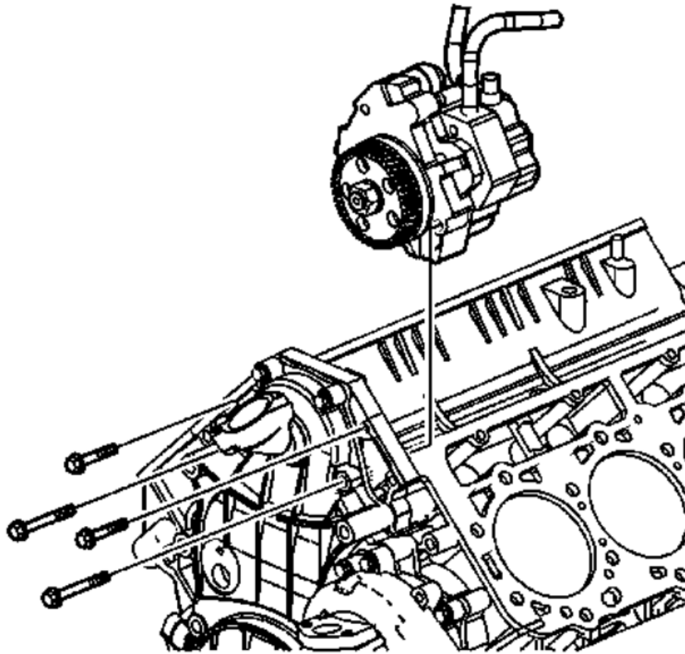
Fig. 13: Install the CP3
