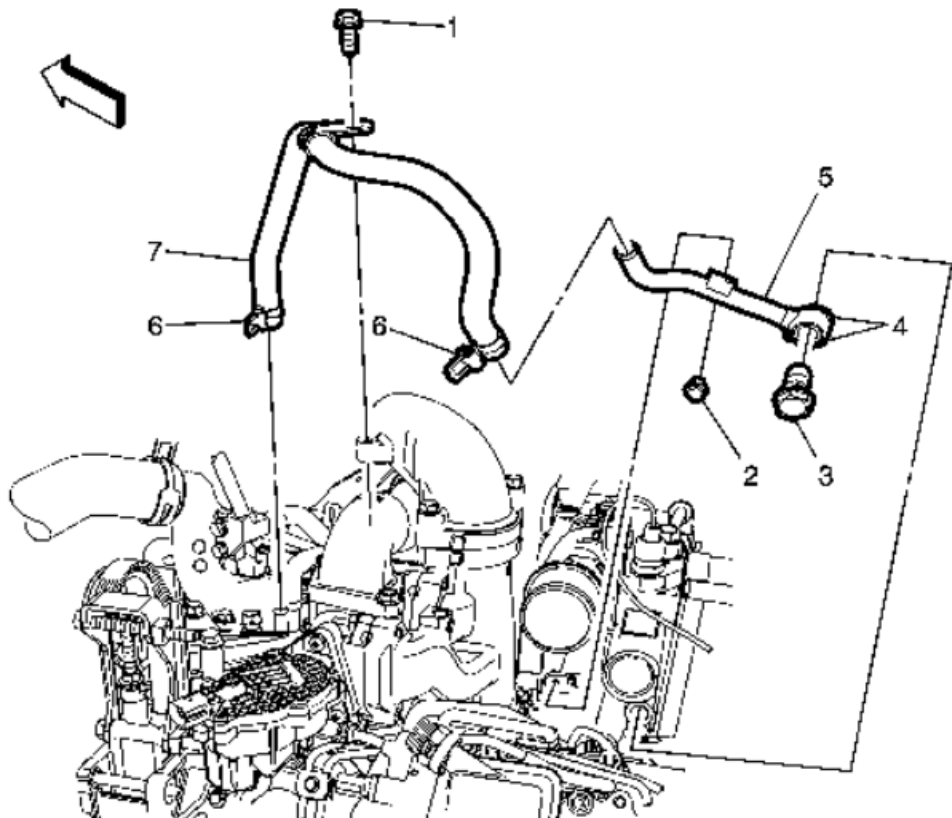
Fig. 7: Turbocharger coolant return pipe removal
