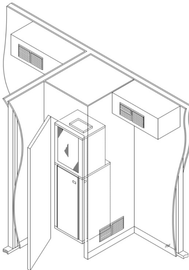
FIGURE 1. Typical Suite Installation
