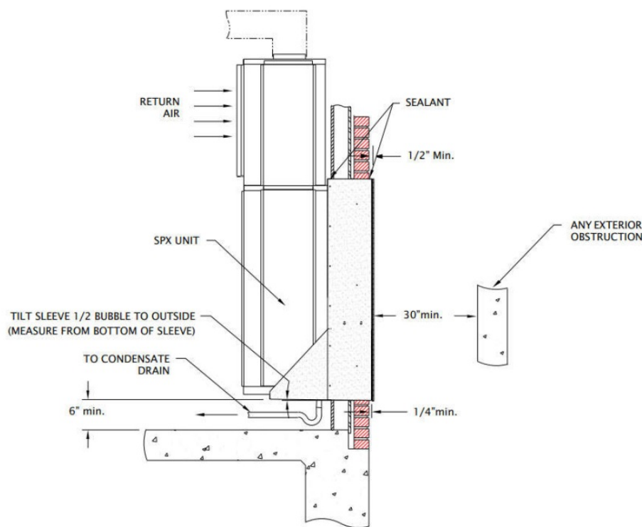
FIGURE 6. Side View
