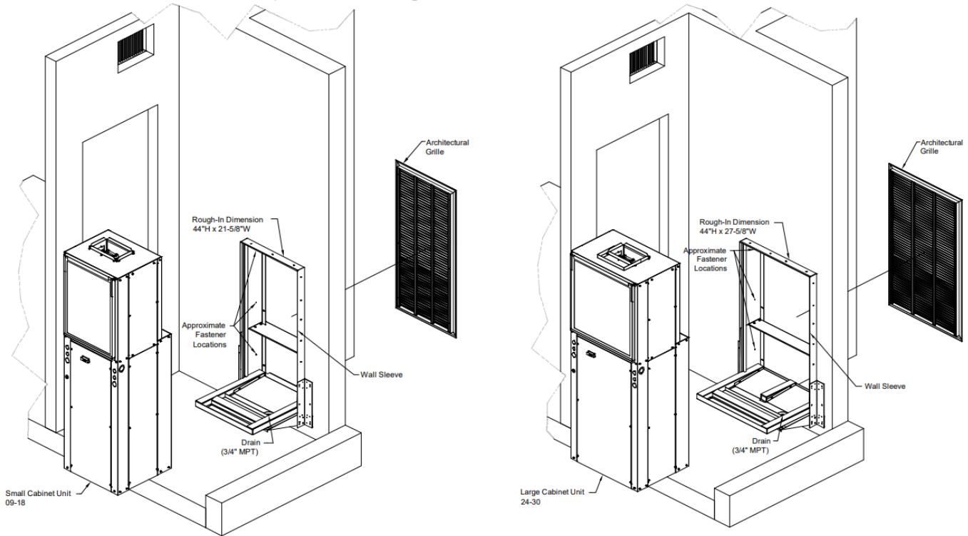
FIGURE 4. General Assembly (Small and Large Sleeve)
