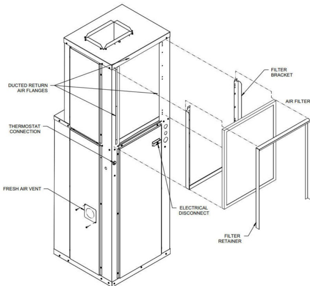
FIGURE 5. Filter Bracket Detail
