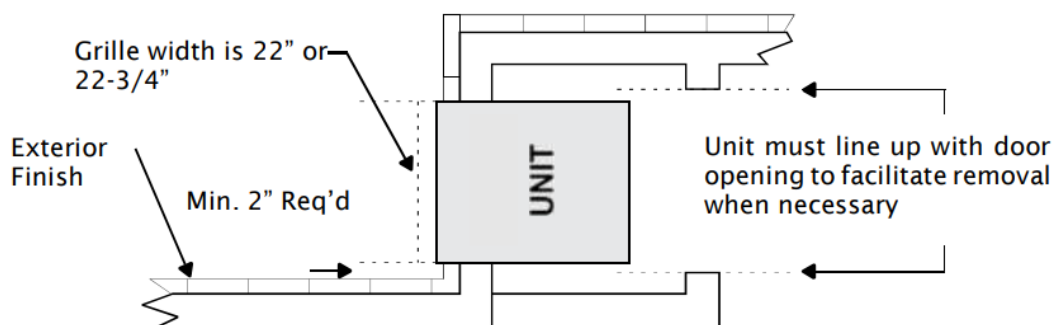
FIGURE 2. Small Sleeve Closet Installation and Dimensions
