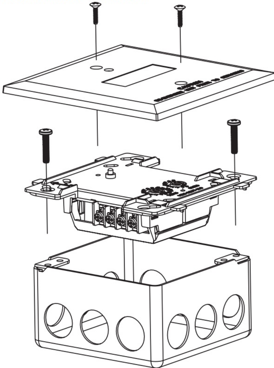
FIGURE 2. MODULE MOUNTING:
