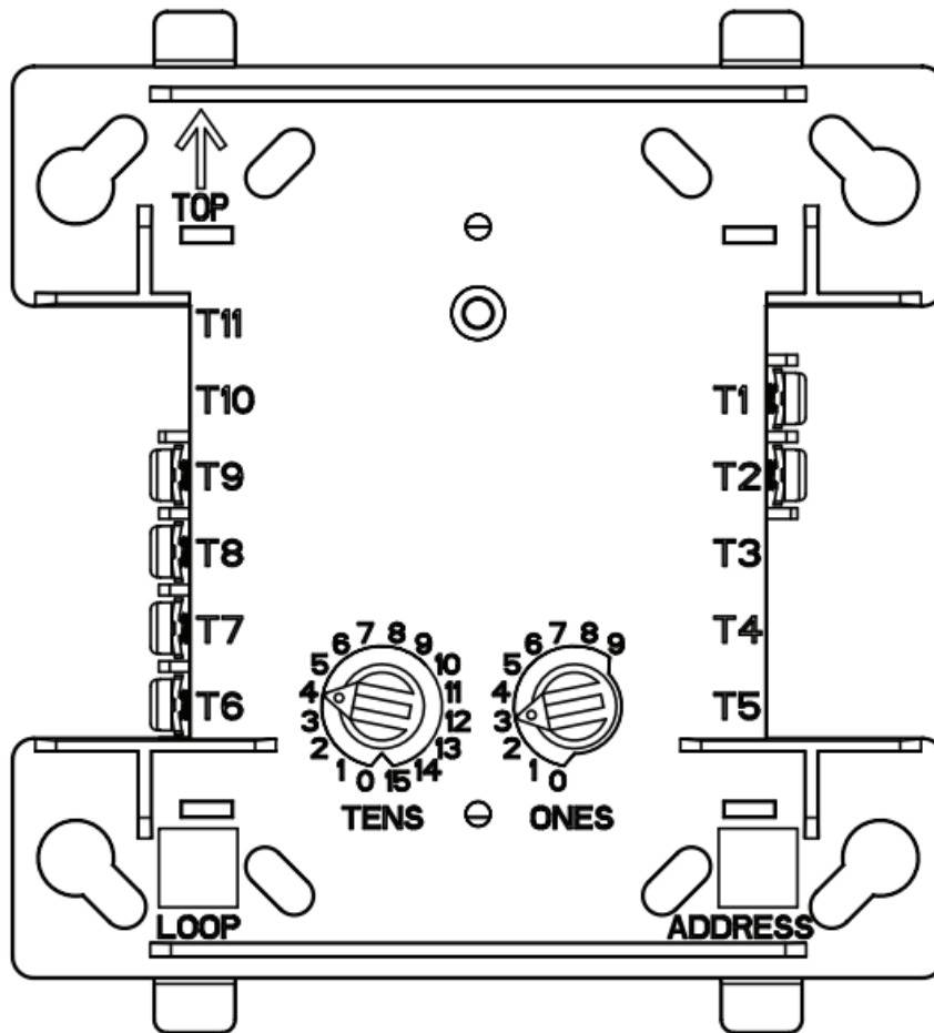
FIGURE 1. REMOVING ROTARY SWITCH STOP:
