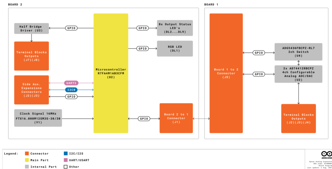
Block diagram
