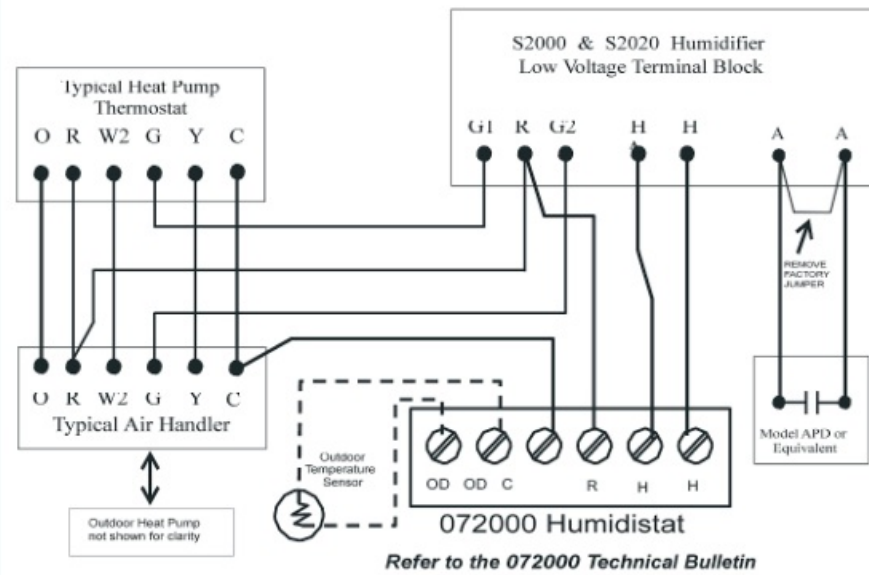
FIG 9 HEAT PUMP SYSTEM AND STEAM HUMIDIFIER WITH 072000 HUMIDISTAT
