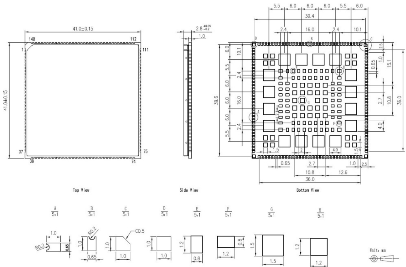
Figure 31. Structure dimensions (unit: mm)
