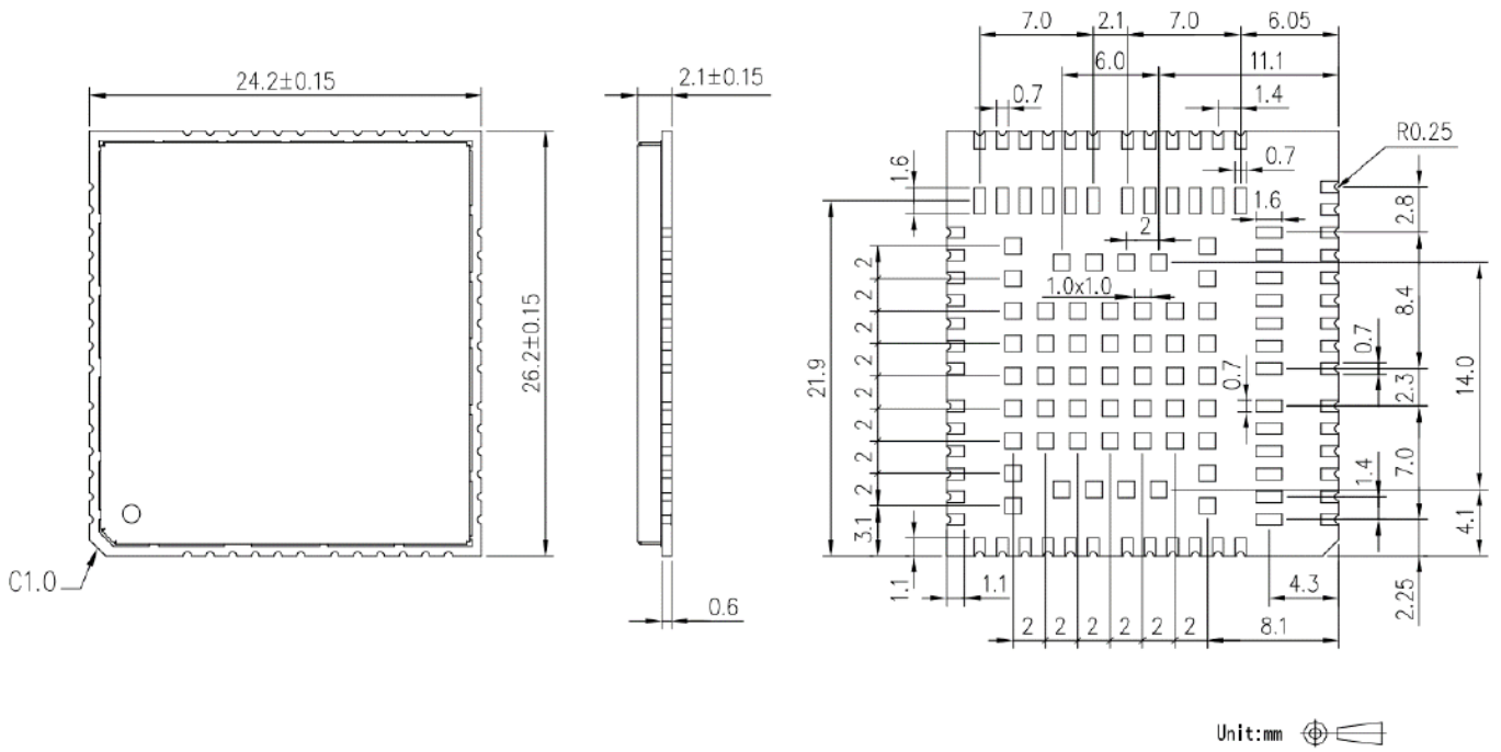
Figure 3. Structural dimension drawing (unit: mm)
