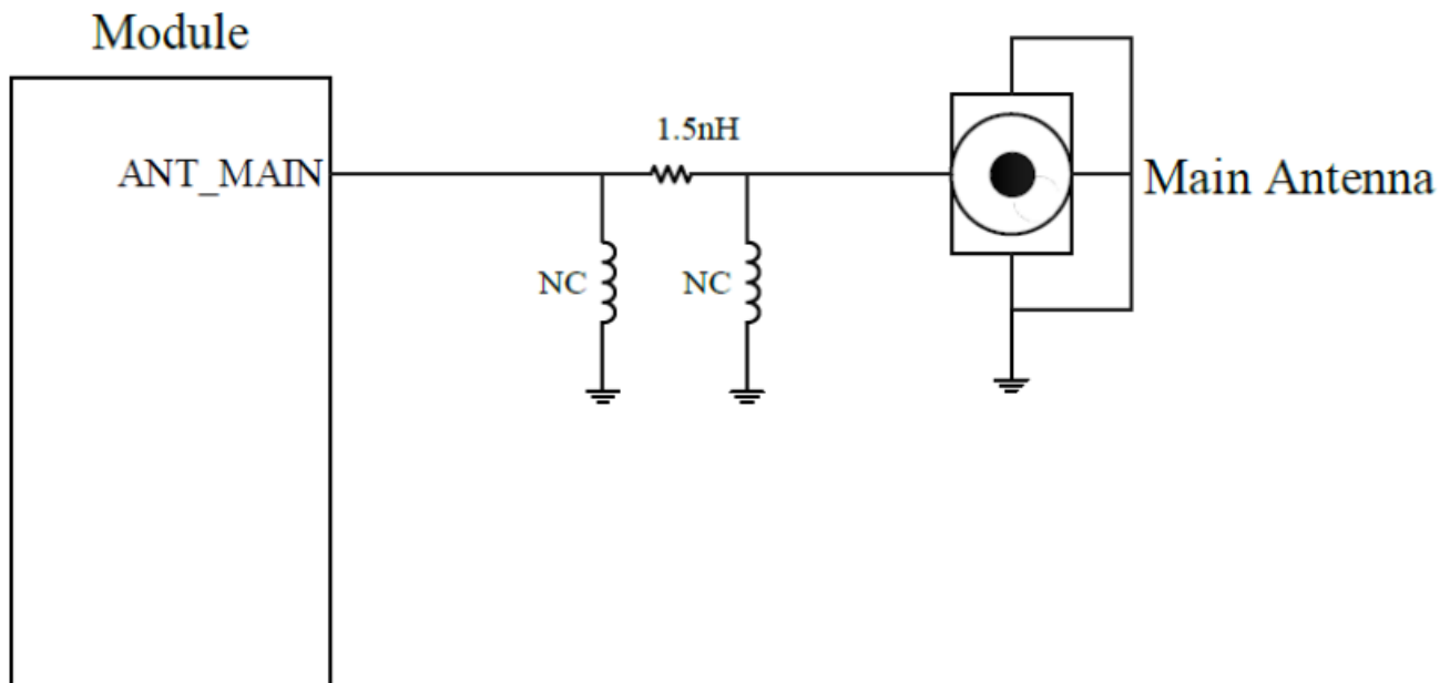
Figure 4. RF reference circuit design
