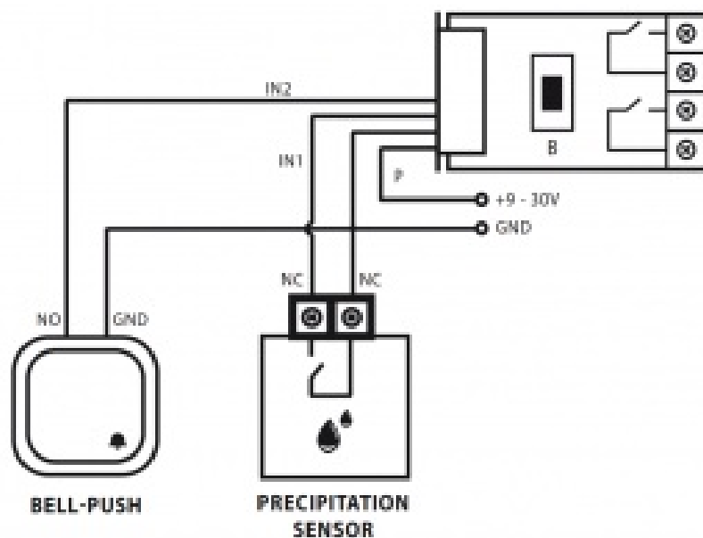
Diagram 5 – example connection to a precipitation sensor
