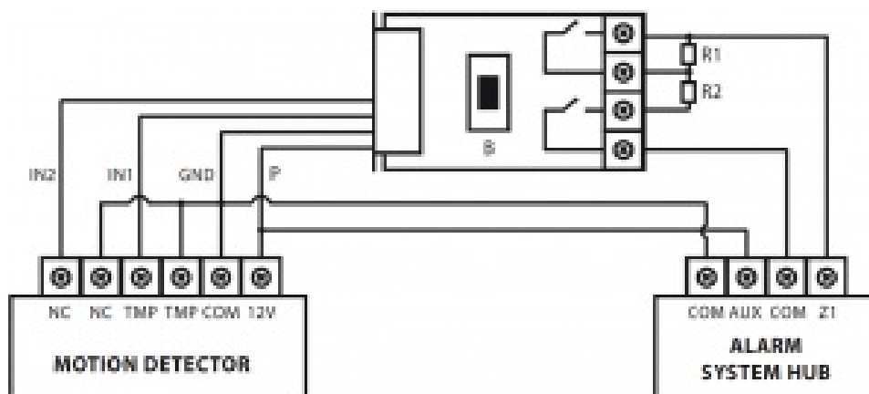
Diagram 3 – Connection to a parametric alarm line
