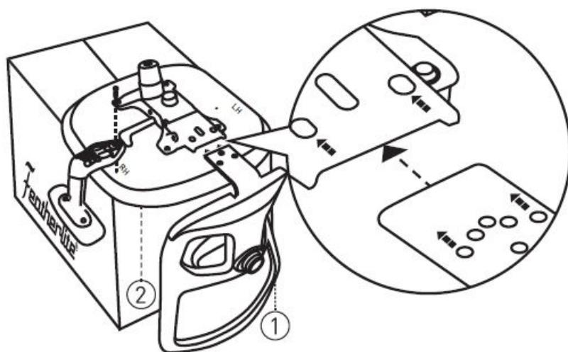
Fix Chair Back to Mechanism Seat
