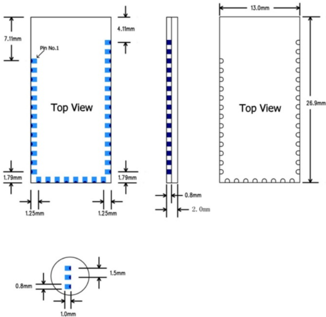
Figure 10: FSC-BW236 footprint
