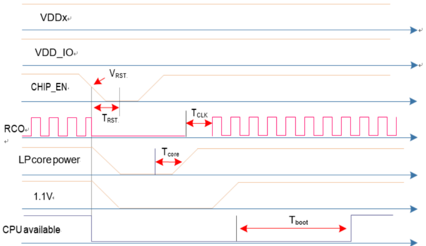
Figure 7: Timing sequence of shutdown
