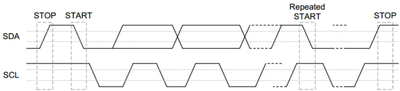
Figure 5: I2C Bus Timing
