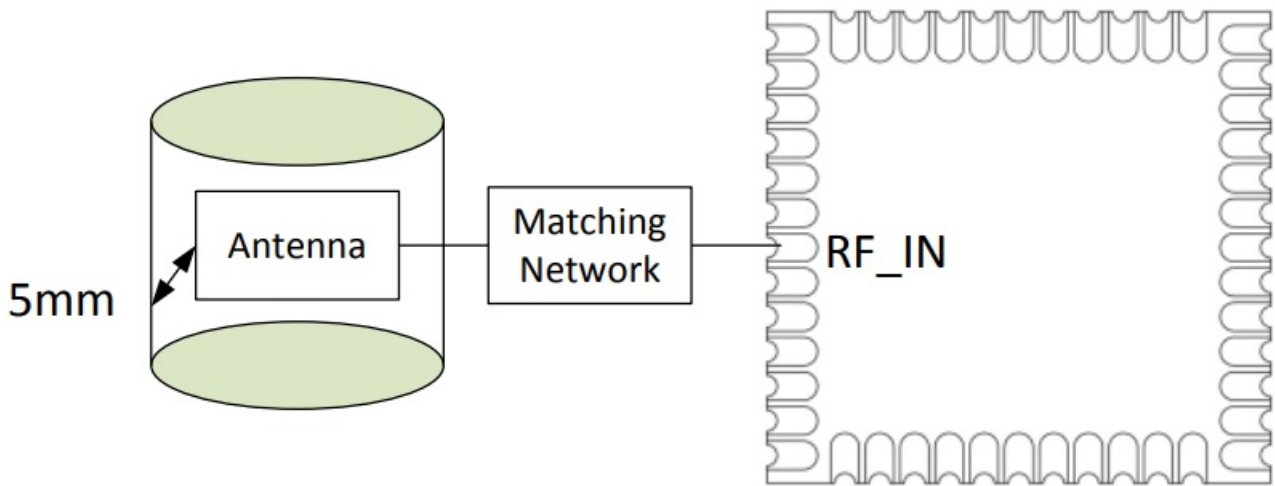
Figure 13: Leave 5mm Clearance Space from the Antenna General design recommendations are:
