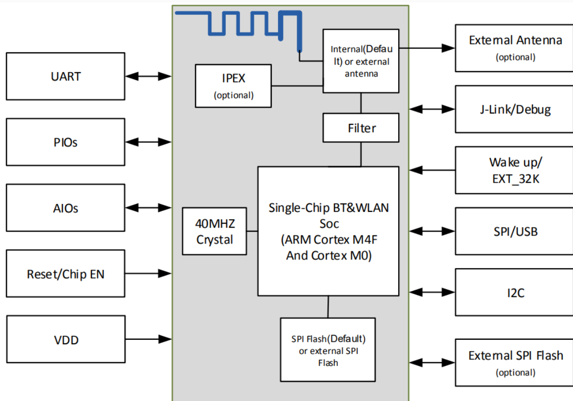
Figure 2: Block Diagram
