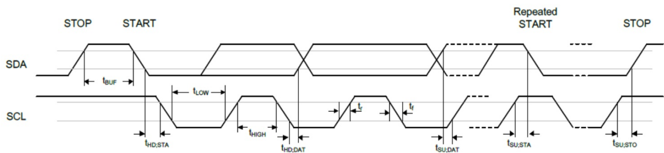
Figure 8: I2C Timing Diagram
