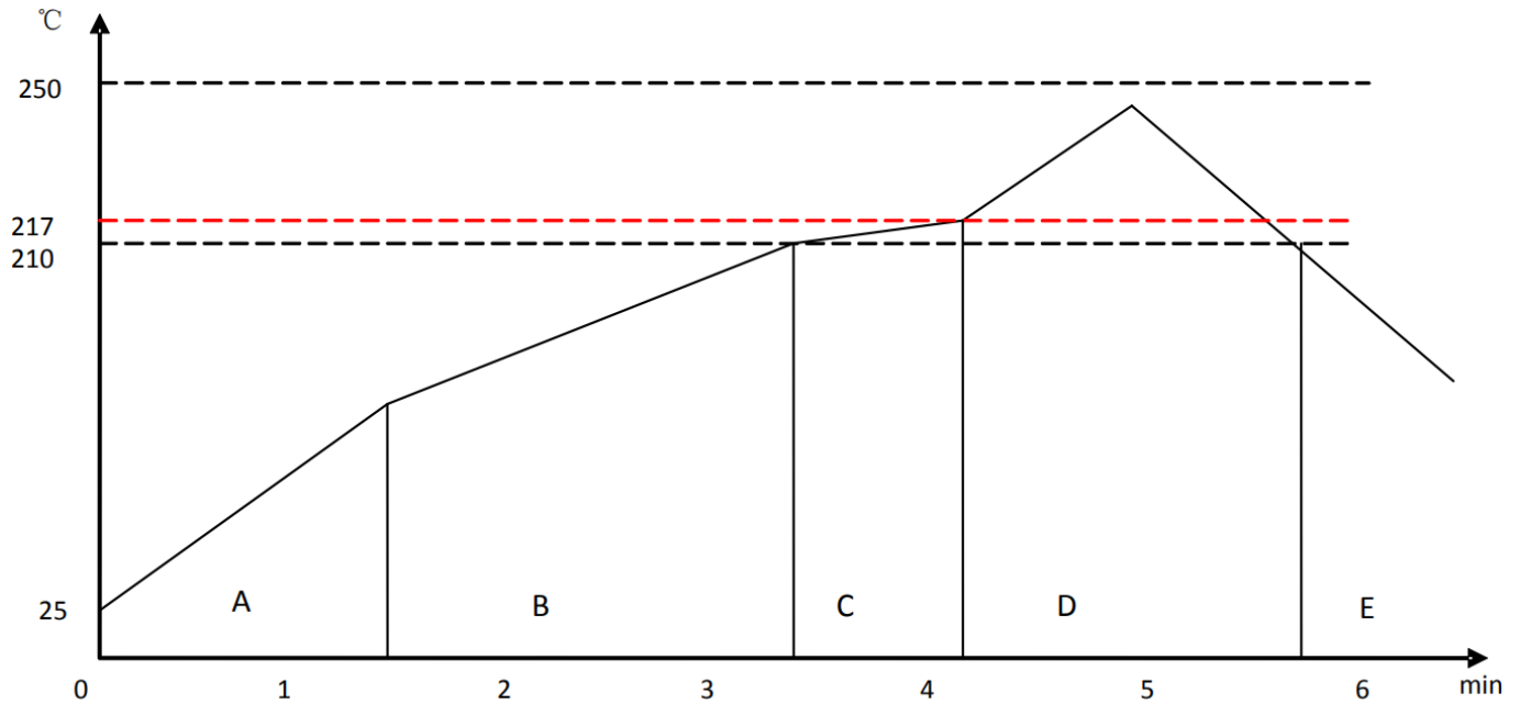
Figure 9: Typical Lead-free Re-flow
