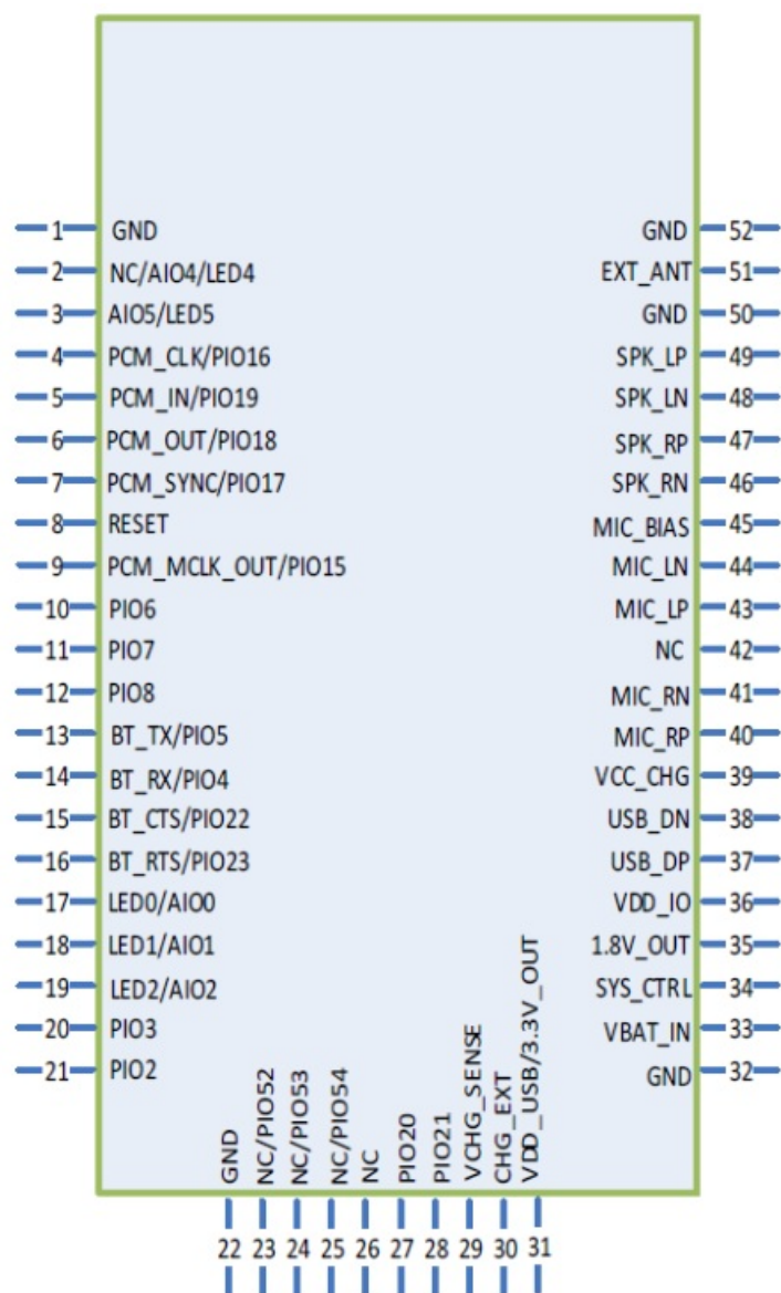
Figure 2: FSC-BT1026D PIN Diagram(Top View)
