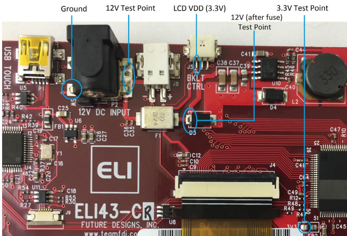
Figure 3. ELI43-CP Power Test Points
