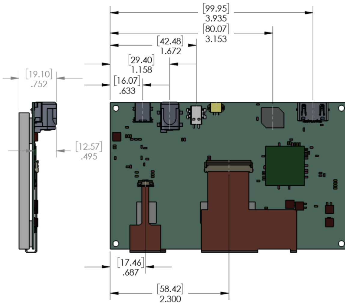
Figure 10. Side and Back Views with Measurements
