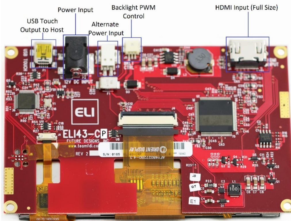
Figure 2. ELI43-CP Connectors
