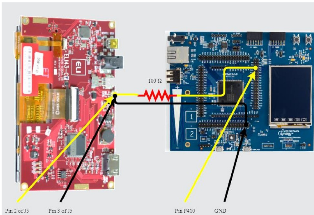
Figure 8. Renesas Synergy S7G2 Signal and Ground
