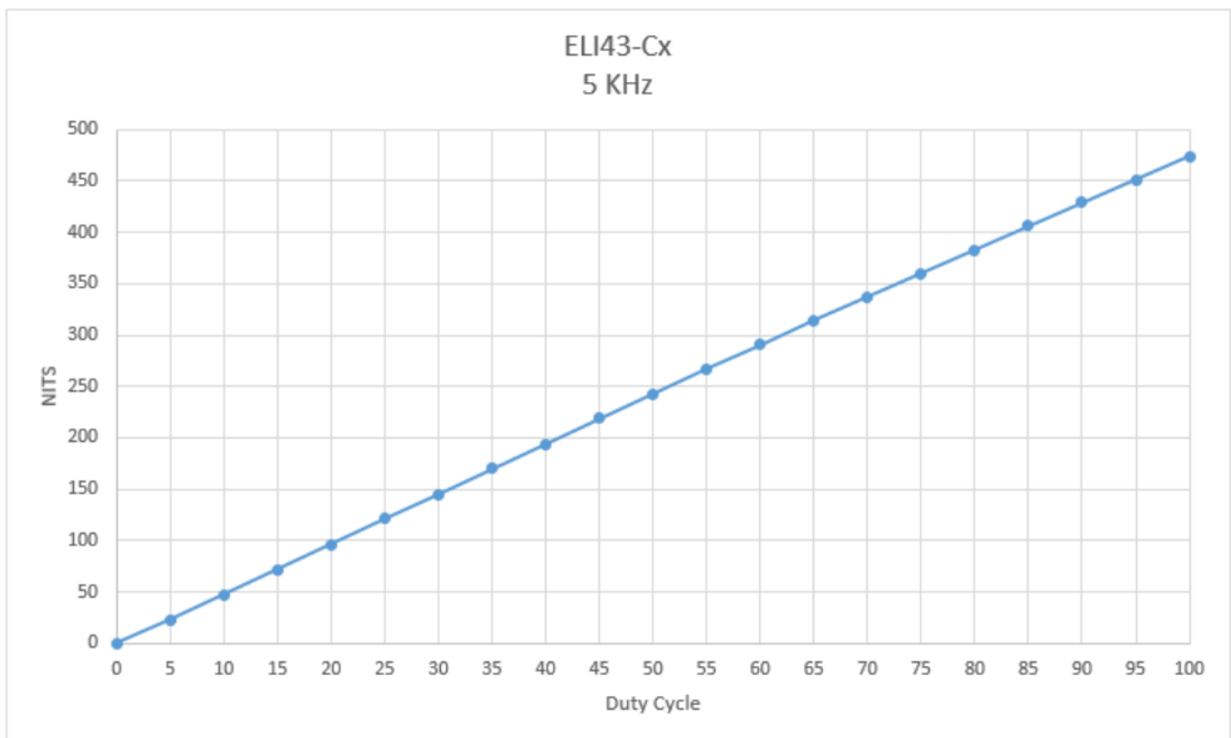
Figure 5. ELI43-CP Backlight Curve in Nits
