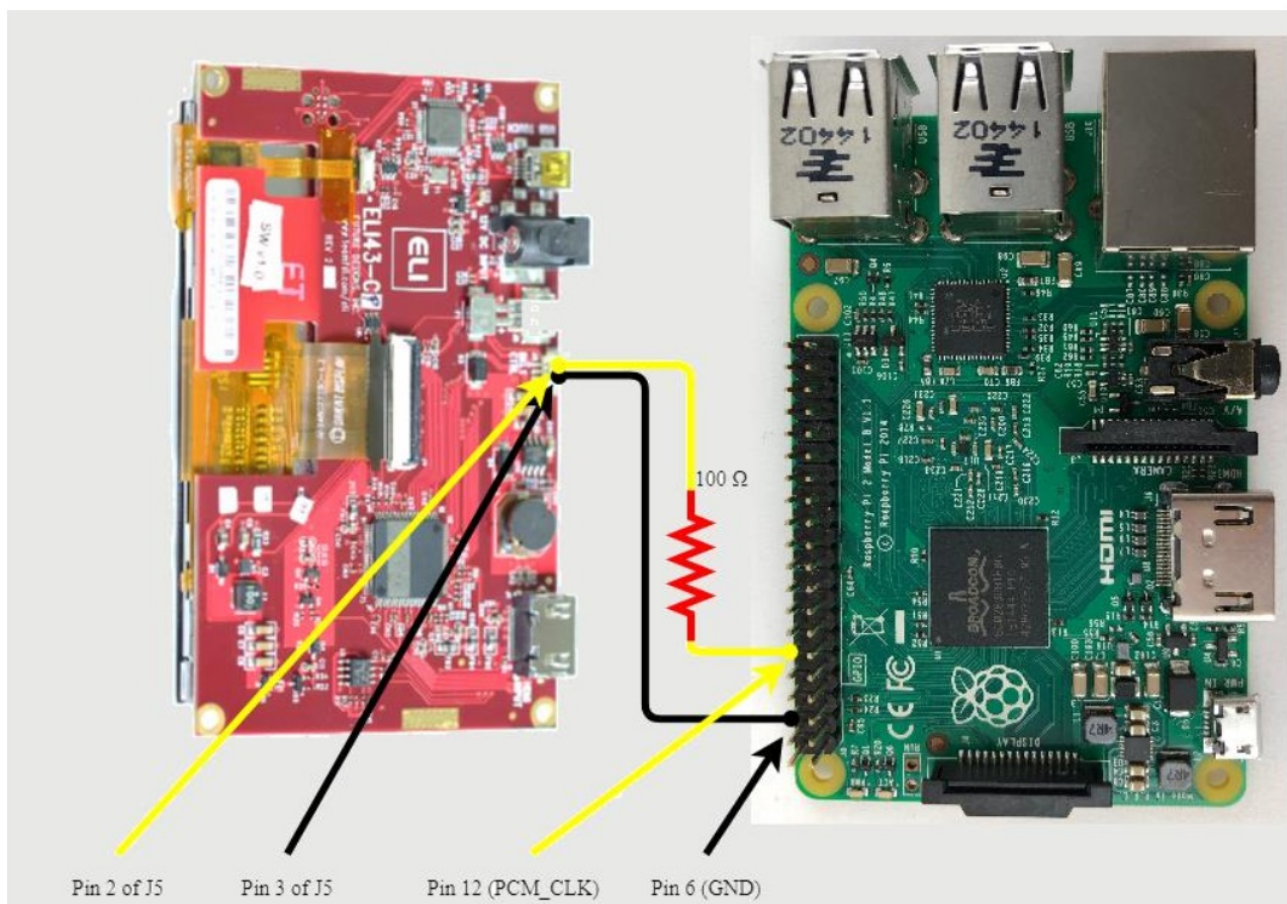
Figure 6. Raspberry Pi Signal and Ground
