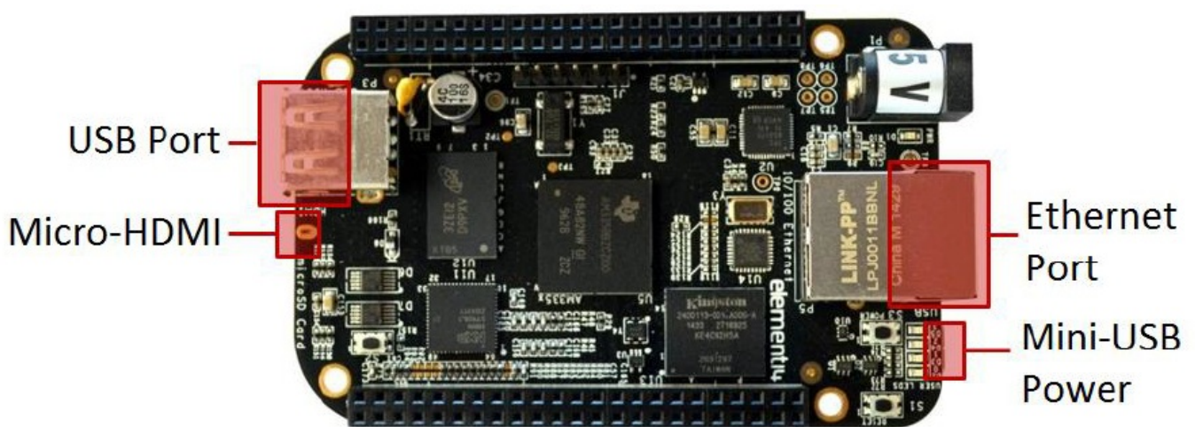
Figure 13. BeagleBone Black Connections
