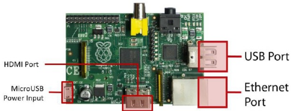
Figure 3. Raspberry Pi Model B Connections
