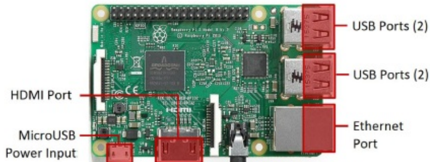
Figure 6. Raspberry Pi 3 Model B Connections
