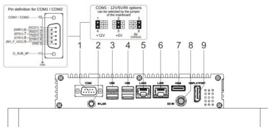
Right side of the Capacitive Touch PC
