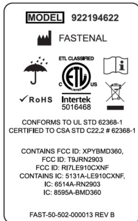
Controller (with cellular data interface)
