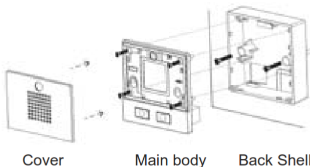
Figure 3-2 Three Major Parts of i10D
