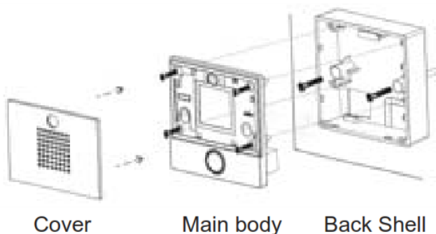
Figure 3-1 Three Major Parts of i10&i10V
