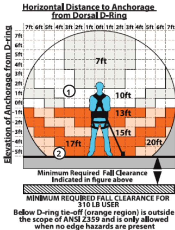
Figure 6 - Arc Flash Mini Pro Minimum Required Fall Clearance for 130 to 310 lbs. (59 to 141 kg) Users
