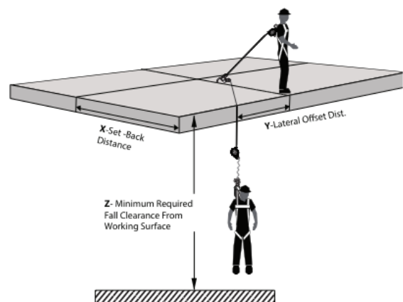
Figure 14 - MRFC Non-Overhead Anchorage
