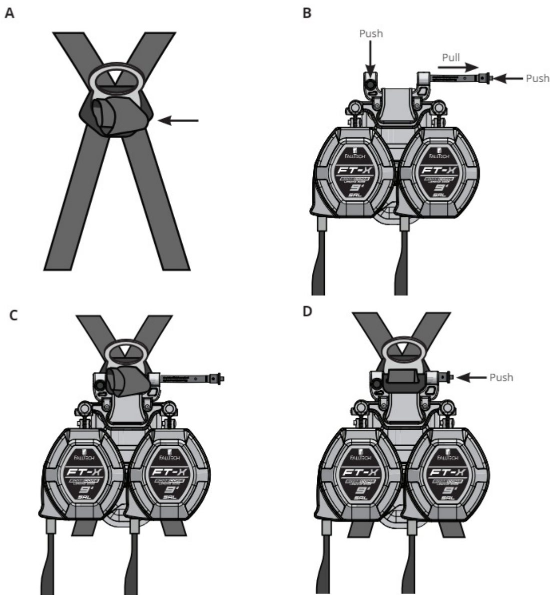
Figure 6 – FT-XTM EdgeCore™ Arc Flash Tie-Back Class 2 Leading Edge SRL-P Installation
