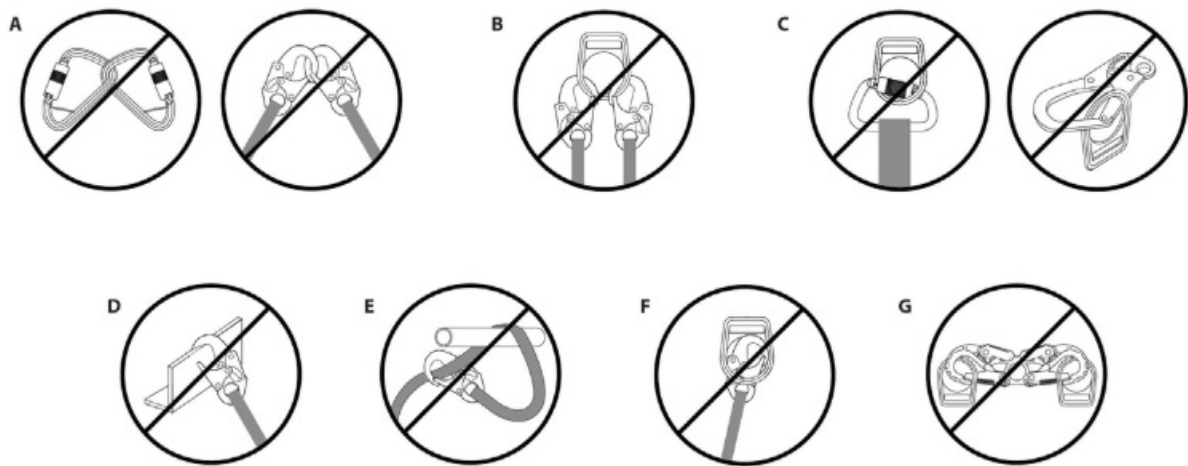
Figure 5 – Non-Compatible Connections
