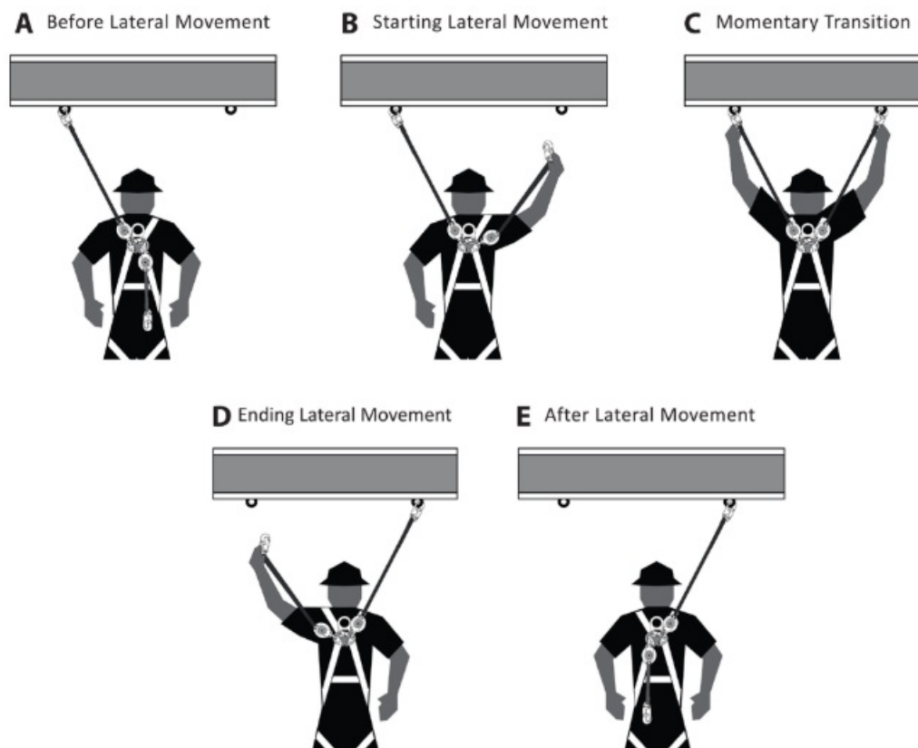
Figure 8 – Twin-Leg SRL-Ps for Lateral Movement
