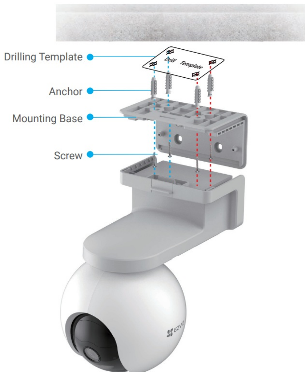
Fig. 1 Ceiling Mount
