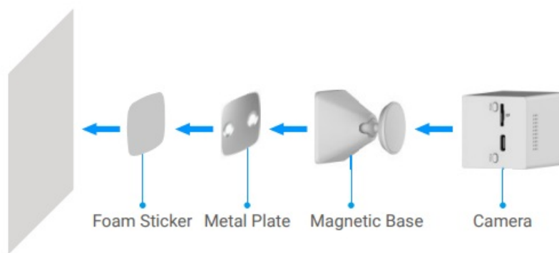
Fig.1 Mount by Foam Sticker
