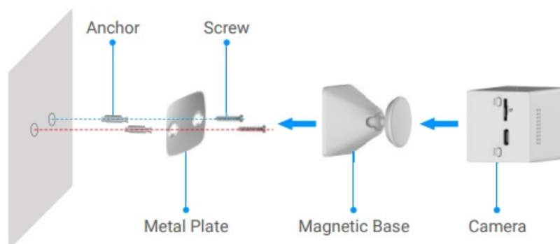
Fig.2 Mount by Screws
