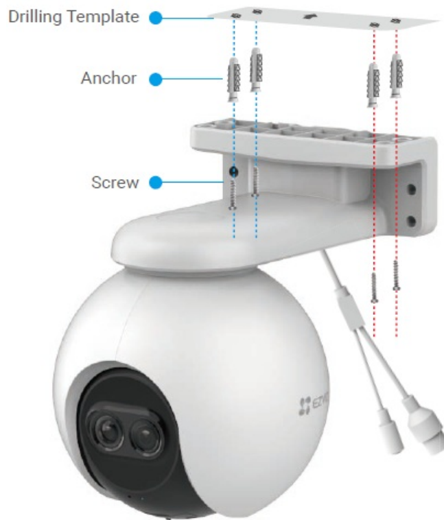
Fig. 1 Ceiling Mount
