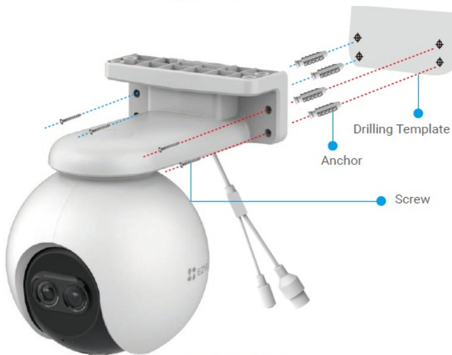
Fig. 2 Wall Mount
