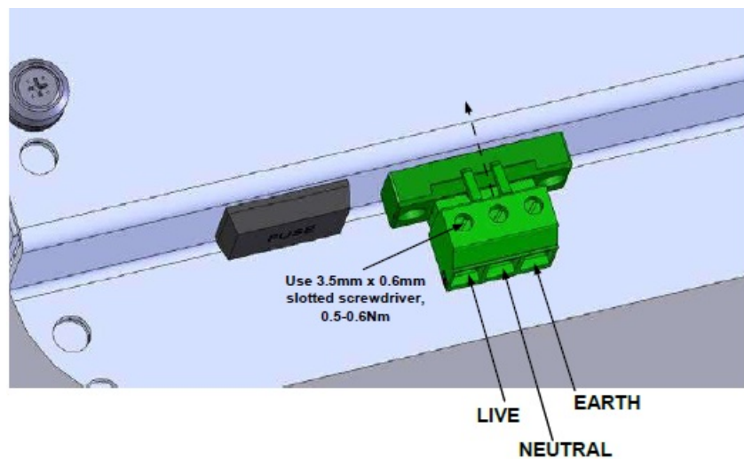
Figure 7: iWAP107 Mains Power Connection
