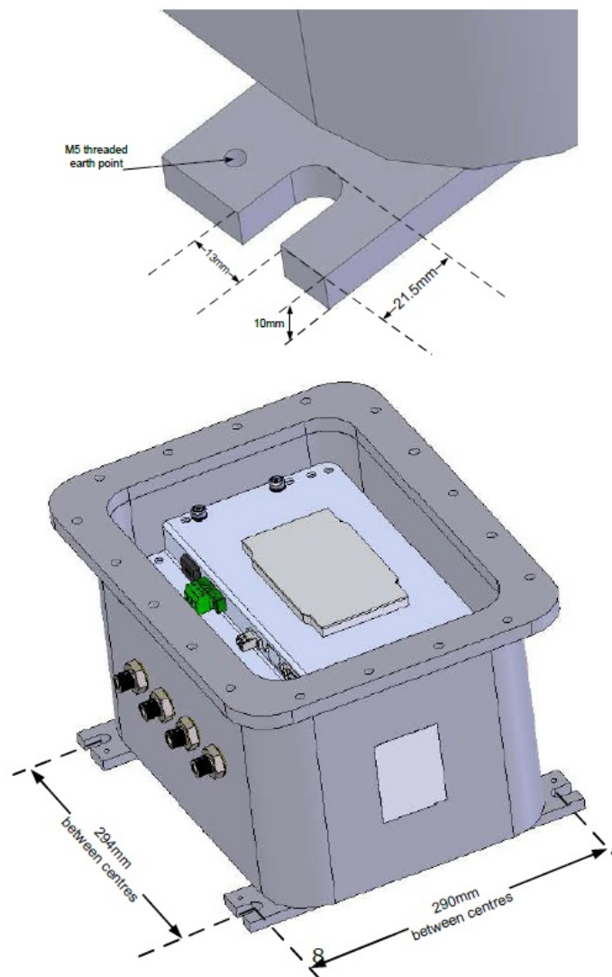
Figure 1: iWAP107 Stainless Steel Enclosure Mounting Points
