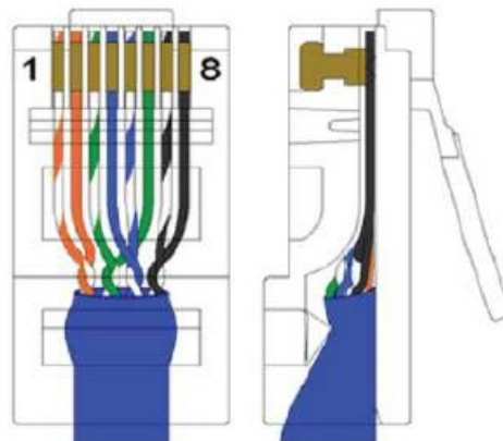
Figure 9: RJ45 CAT5E EIA 568B Plug Wiring
