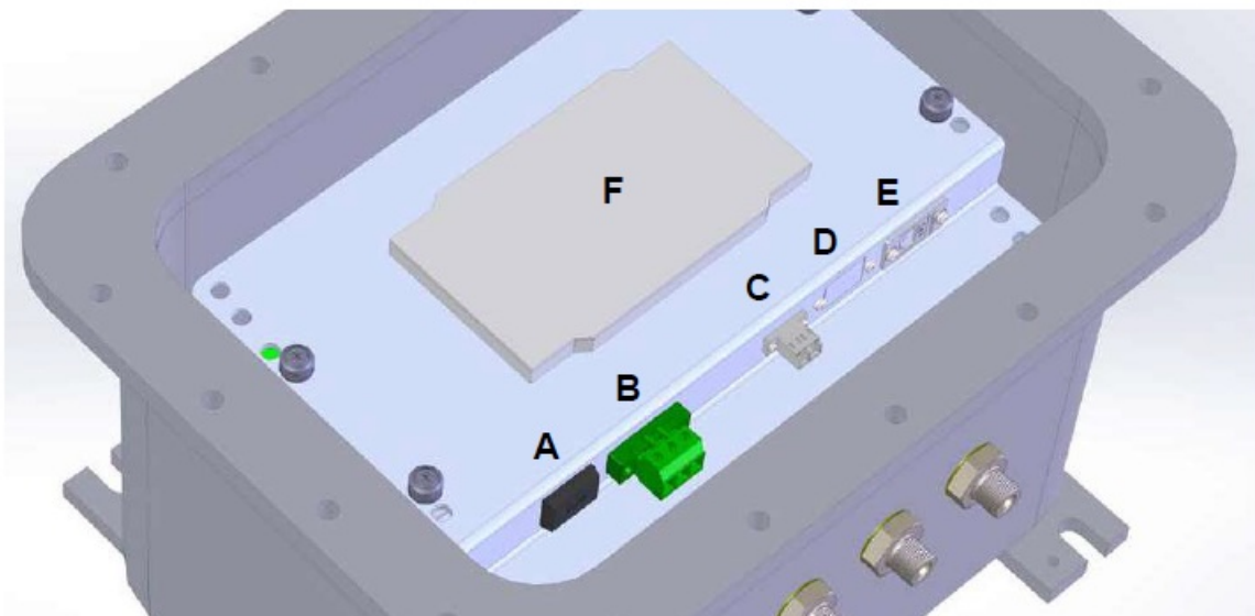
Figure 6: iWAP107 Internal Connections Showing All Options
