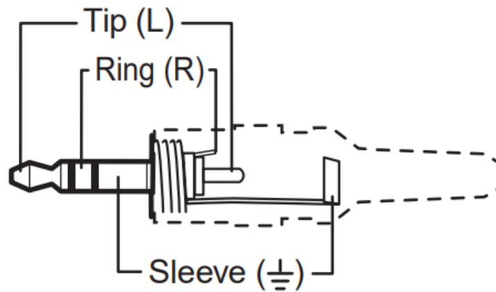
Figure 11. 3.5 mm stereo audio plug
