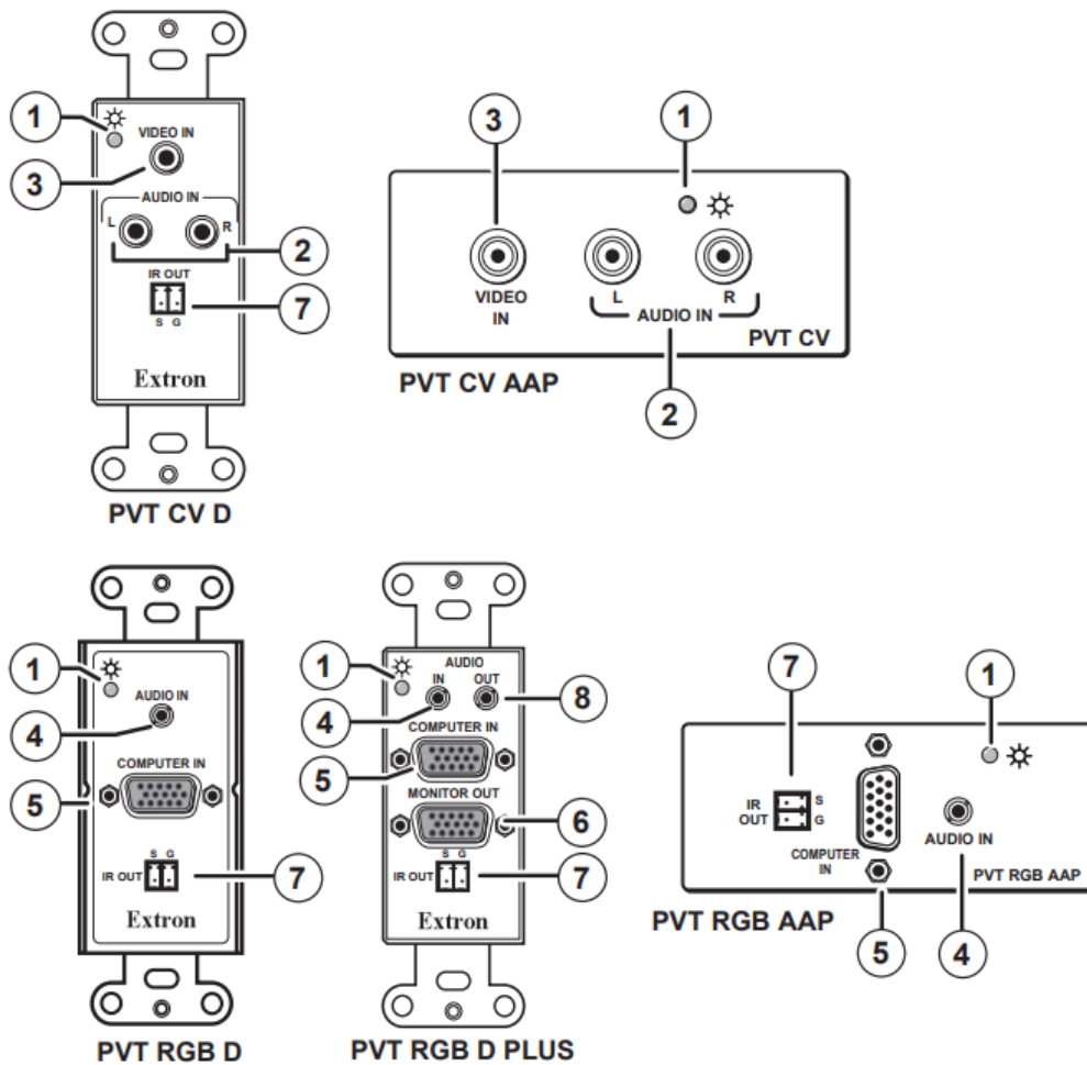
Figure 9. PVT series front panel features
