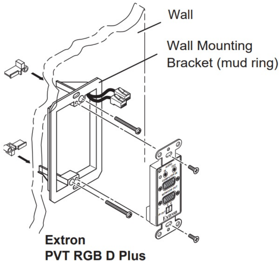
Figure 7. Installing the mud ring
