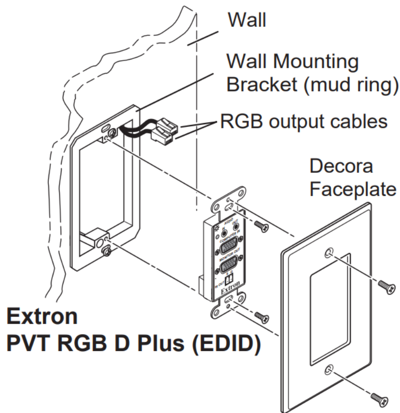
Figure 16. Mounting the PVT RGB D Plus (EDID)
