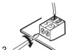
Figure 13. Connecting the PVT CV D to the PoleVault switcher
