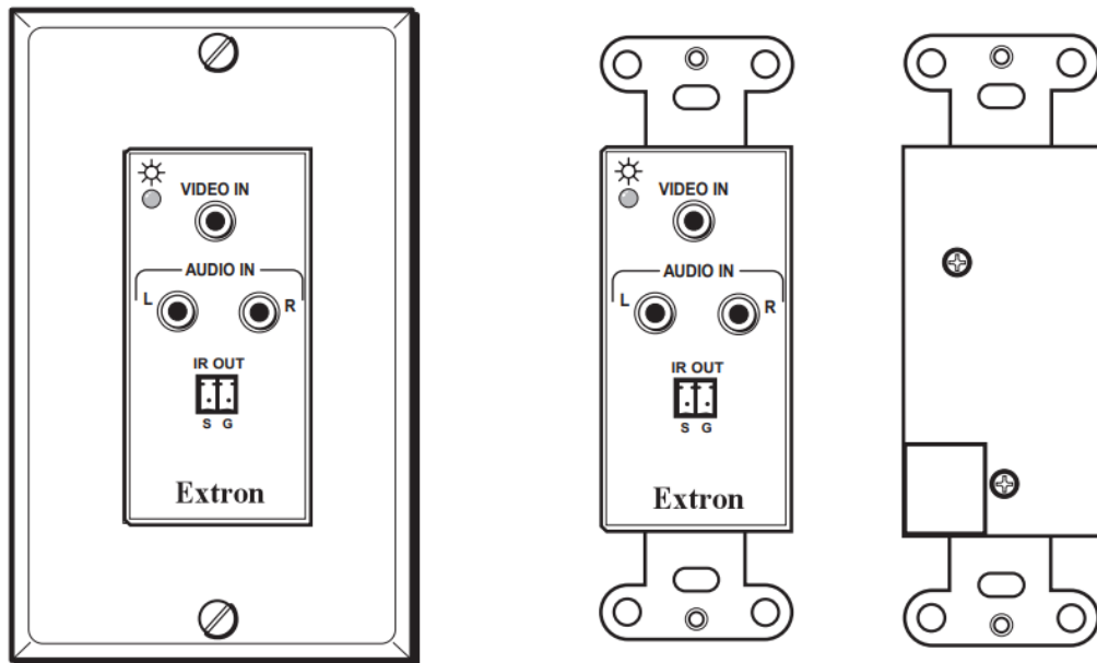
Figure 1. PVT CV D face and rear panels
