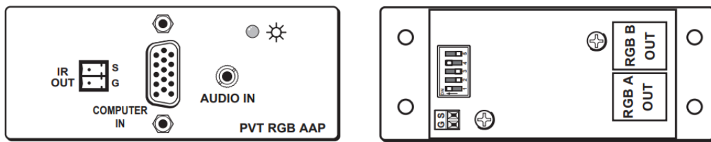
Figure 5. PVT RGB AAP face and rear panels
