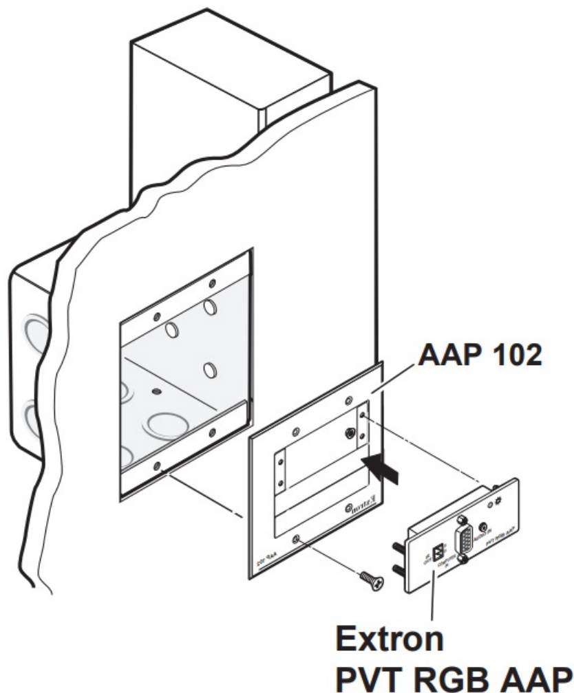
Figure 8. Mounting the PVT RGB AAP
