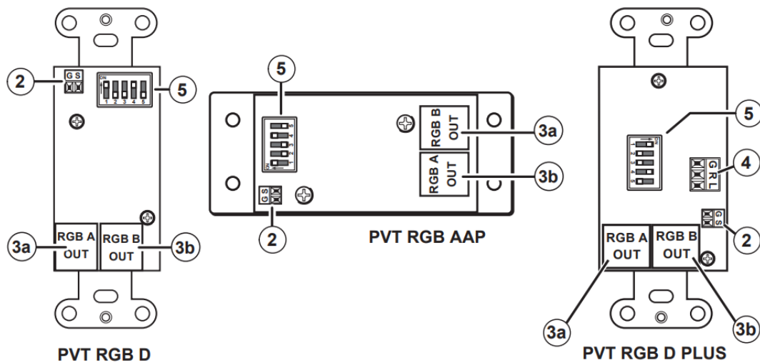
Figure 14. PVT RGB models rear panel features
