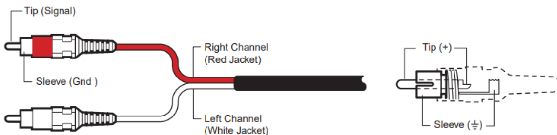
Figure 10. RCA audio connectors
