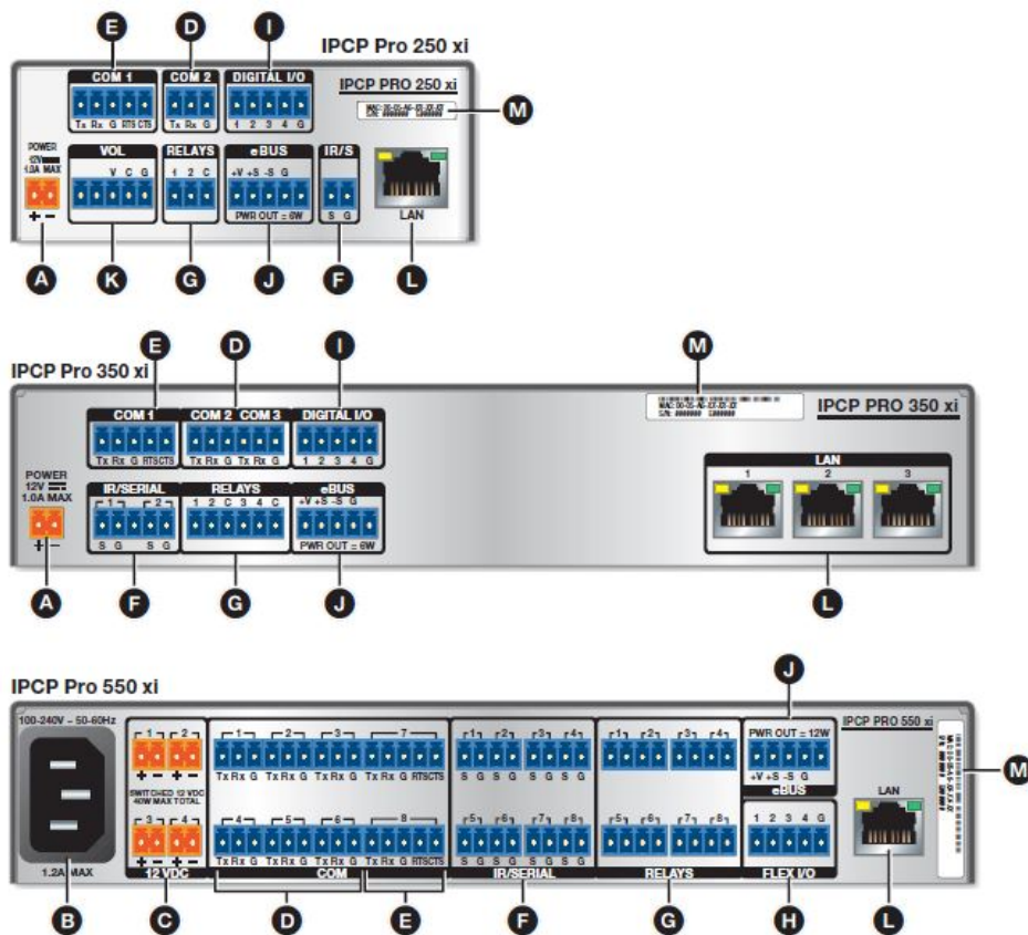
Figure 4. IPCP Pro xi Control Processors —Rear Panels
