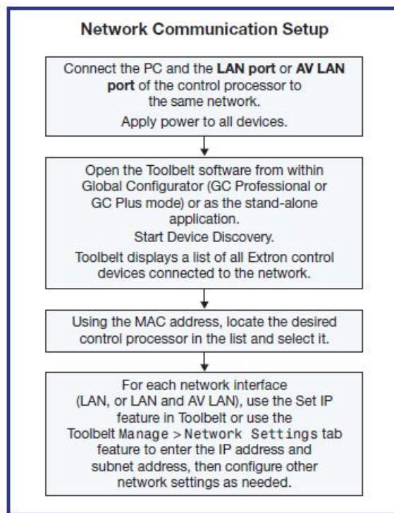
Figure 1. Network Setup
