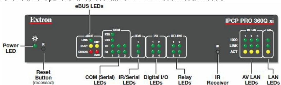
Figure 3. IPCP Pro 360Q xi Front Panel
