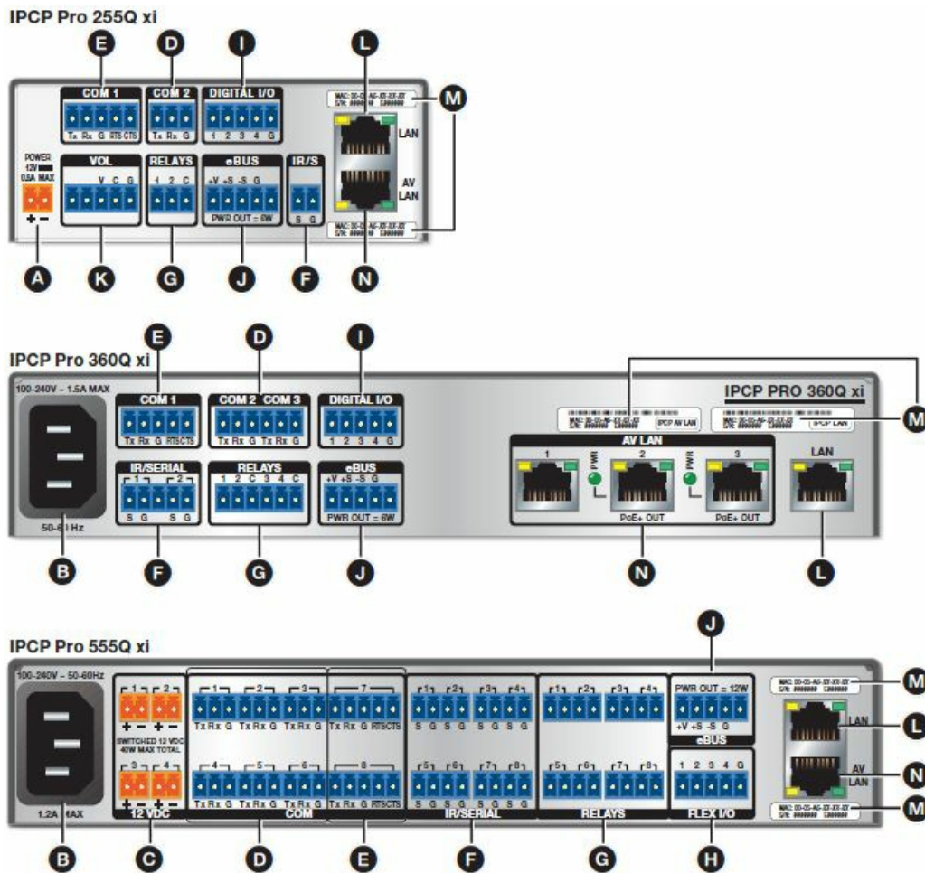
Figure 5. IPCP Pro Q xi Control Processors — Rear Panels
