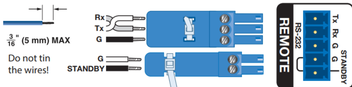
Figure 5. Remote Volume Control and Standby Ports
