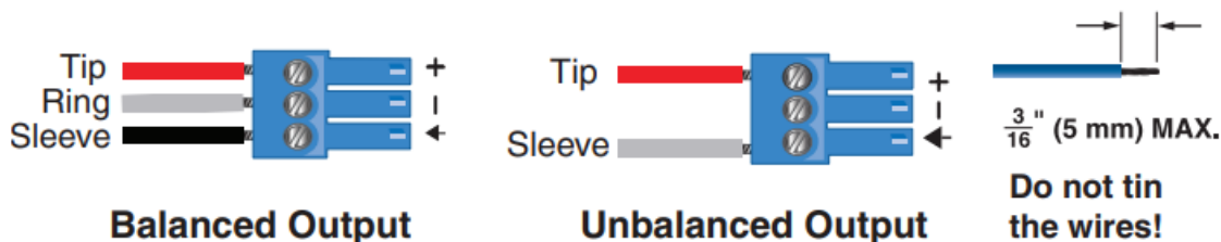
Figure 4. Output Wiring
