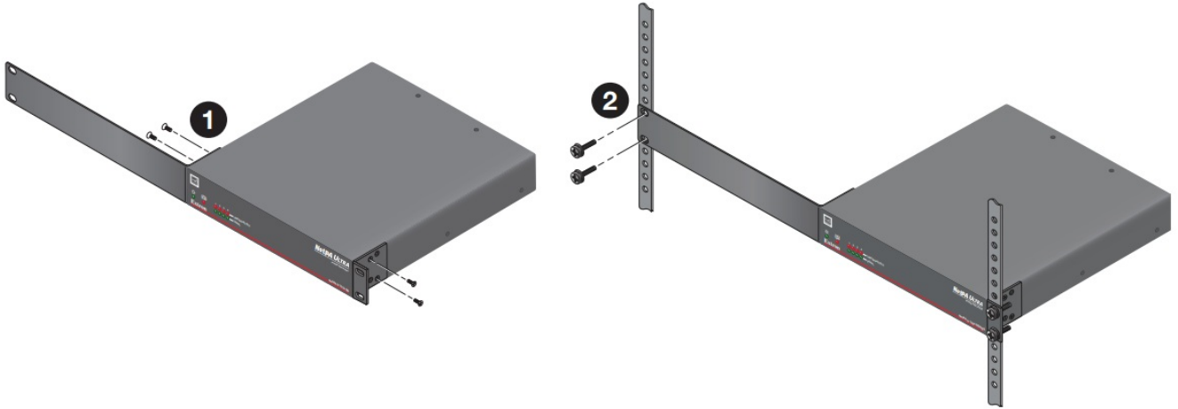
Figure 1. NetPA U 1004 Rack Ear Mounting
