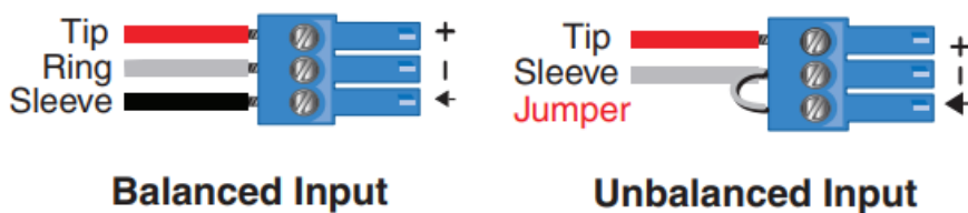
Figure 3. Input Wiring
