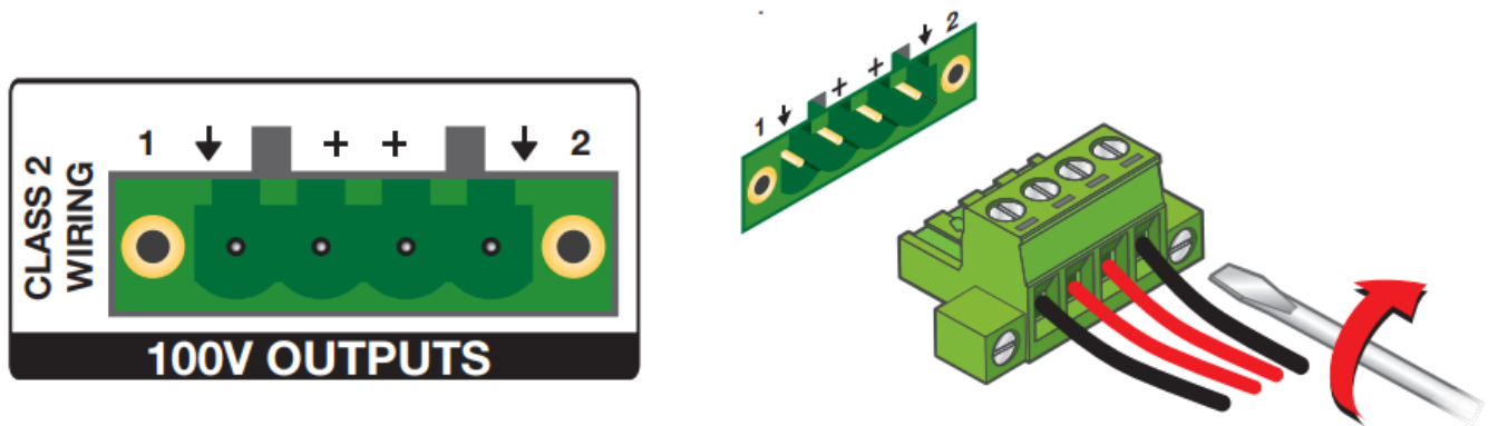
Figure 6 Speaker Output Port and Wiring Diagram
