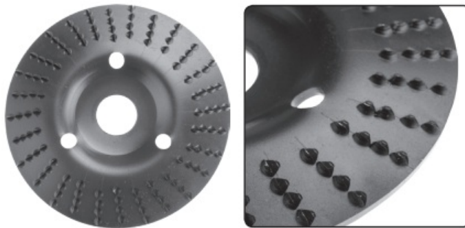
Fig.10, Rasping discs
