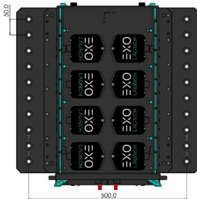
Figure 6: Mounting interfaces of the 4U TestPod
