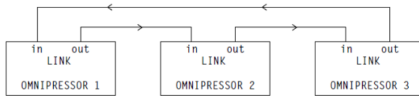
MULTI-UNIT LINKING---BLOCK DIAGRAM
