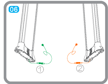
06 Select the bottom of one side of the left or right foot cover to access the power cable
