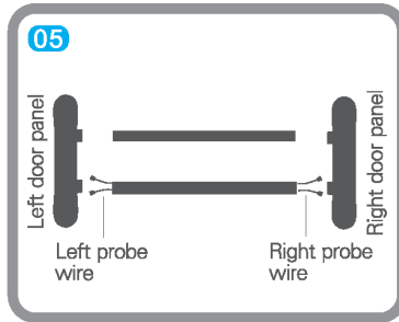
05 Connect the control box cables on the crossbar to the left and right door panels.
